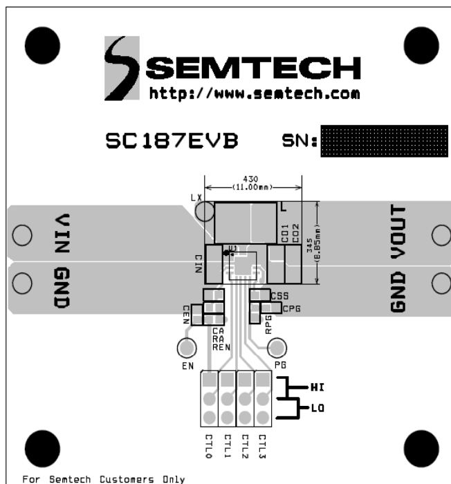
Figure 2 — Recommended PCB Layout (Top Layer)
