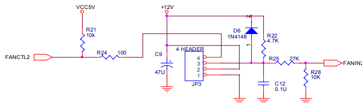
(4 PIN FAN Control) PWM FAN 2 SPEED CONTROL The C11 is reserved for FAN noise dis-bounce.
