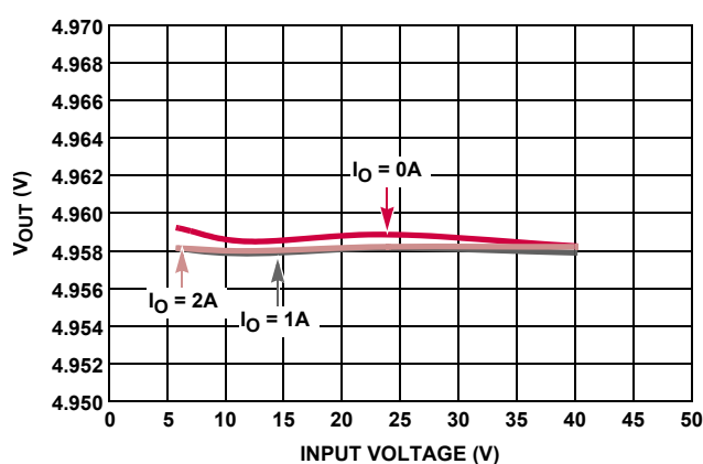
FIGURE 6. LINE REGULATION, V_{OUT} 5V, T_A = +25^\circ\text{C}
