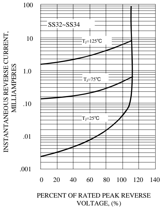
FIG. 3A - TYPICAL REVERSE CHARACTERISTICS
