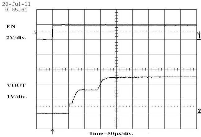
Figure 15. Enable Turn-On (100 \mu\text{A} Load)
