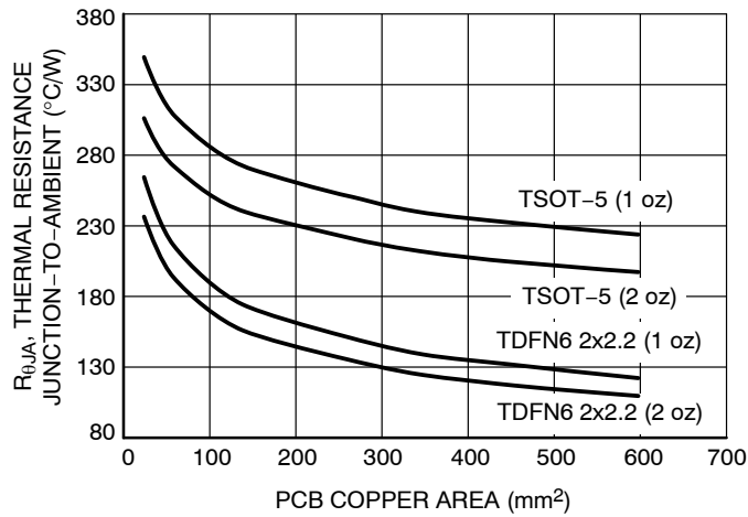
Figure 26. R θJA vs. PCB Copper Area
