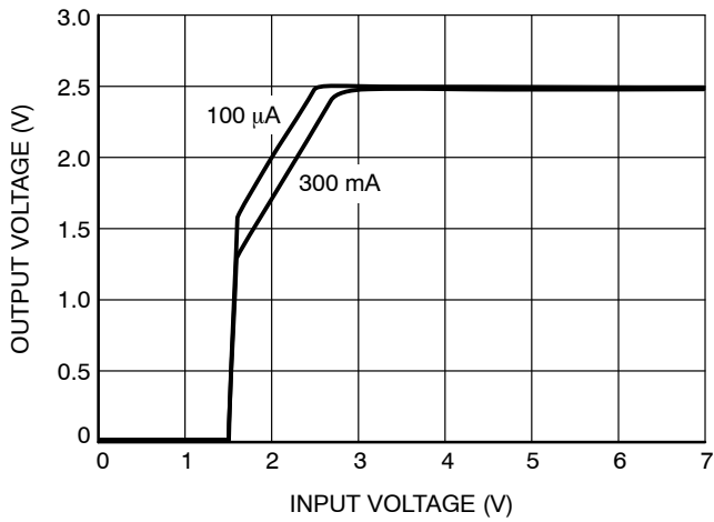
Figure 3. Dropout Characteristics
