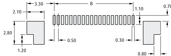
Recommended PC Board Pattern
