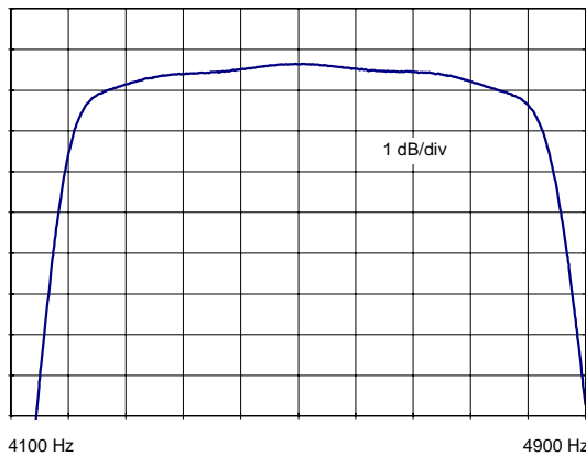
Passband Amplitude
