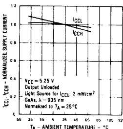
Normalized Supply Current vs Ambient Temperature
