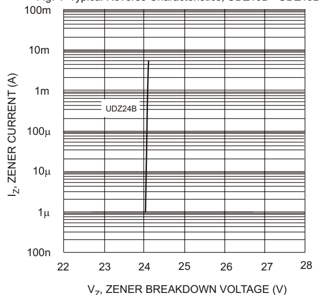
Fig. 6 Typical Reverse Characteristics, UDZ24B
