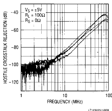
4 × 4 Crosspoint, All Hostile Rejection
