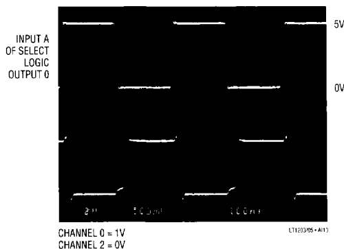
4 × 4 Crosspoint, Switching Channel 0 to Channel 2
