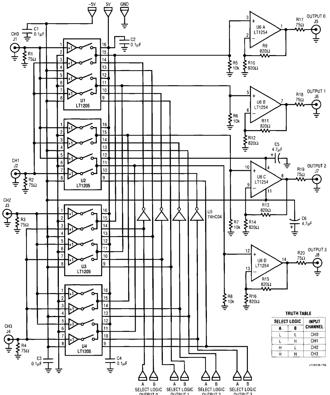
Figure 6. 4 x 4 Crosspoint and Truth Table
