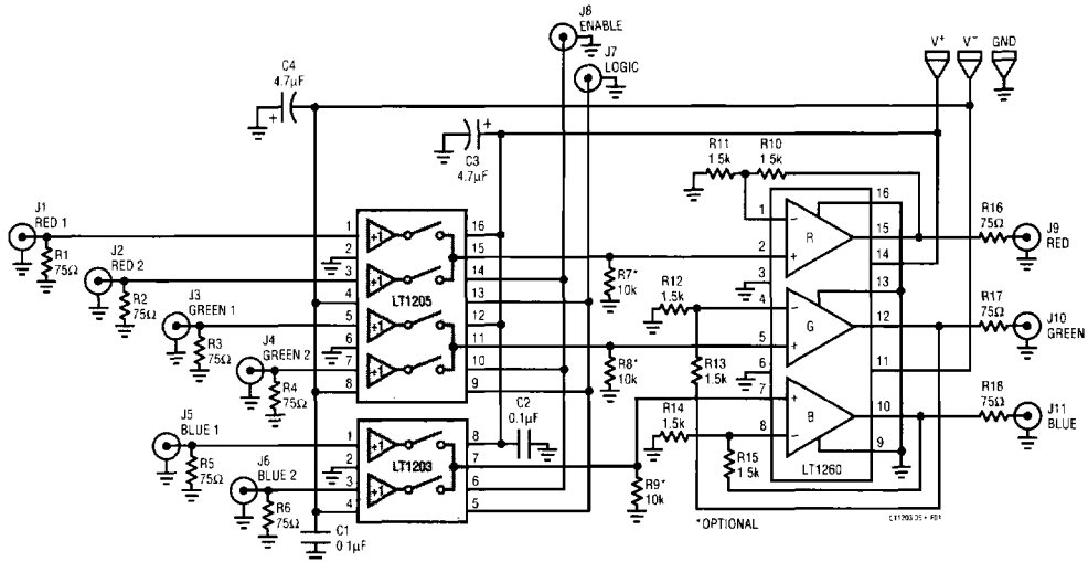
Figure 1. RGB MUX
