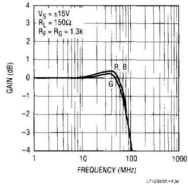
Figure 4. RGB MUX Frequency Response of Demonstration Board #041
