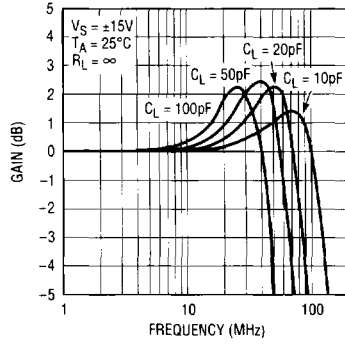
Frequency Response with Capacitive Loads
