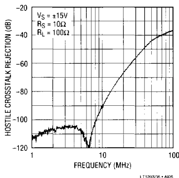
16-to-1 Multiplexer All Hostile Crosstalk Rejection
