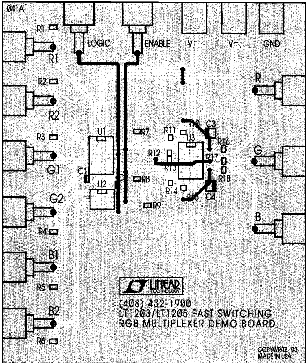
Figure 3. Demo Board #041 Layout
