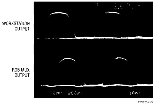
Figure 2a. Workstation and RGB MUX Output
