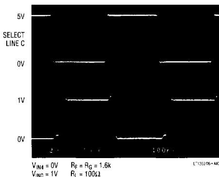
16-to-1 MUX, Switching LT1205 Enable Lines
