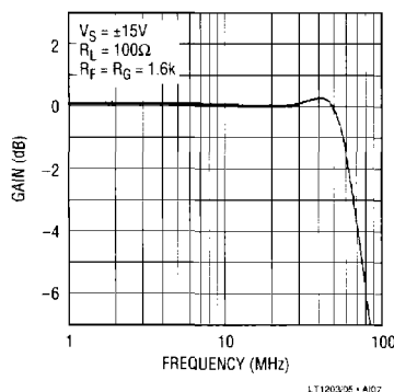
16-to-1 MUX Response
