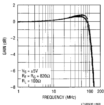
Response of All Four Inputs for the 4 × 4 Crosspoint
