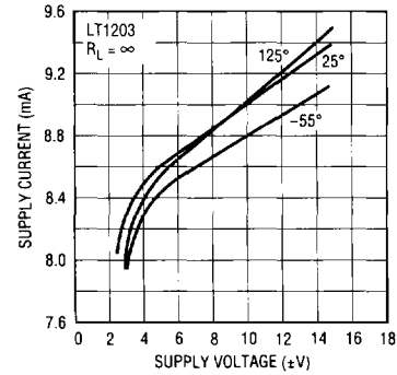
Supply Current vs Supply Voltage (Enabled)
