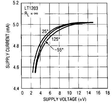
Supply Current vs Supply Voltage (Disabled)
