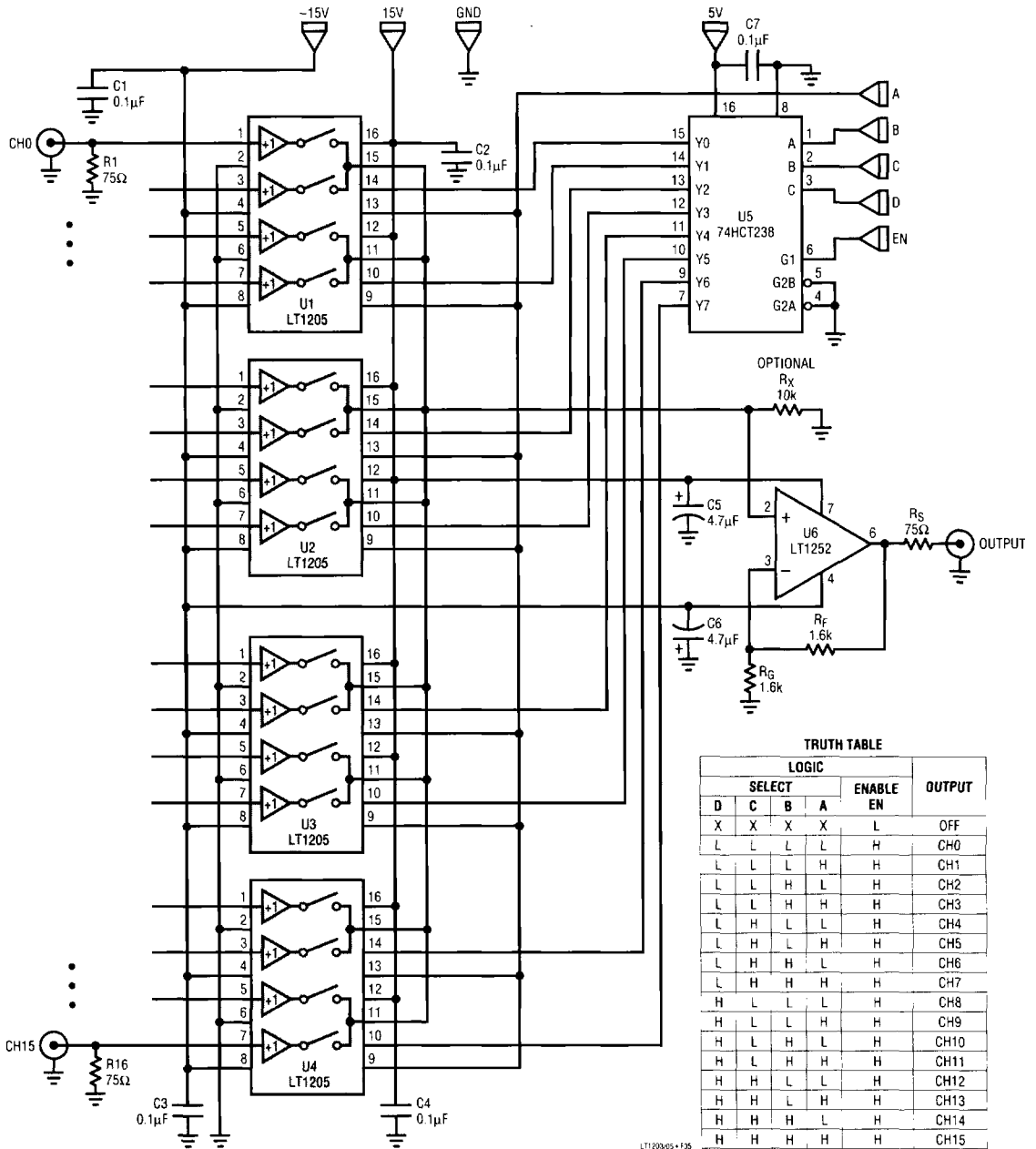
Figure 5. 16-to-1 Multiplexer and Truth Table
