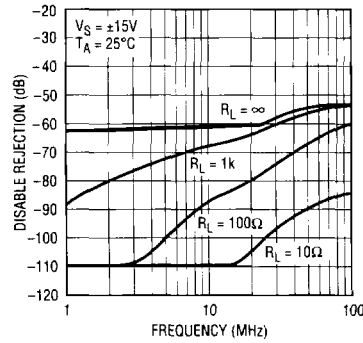
Disable Rejection vs Frequency
