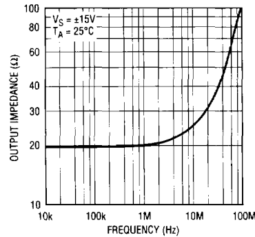
Output Impedance (Enabled) vs Frequency
