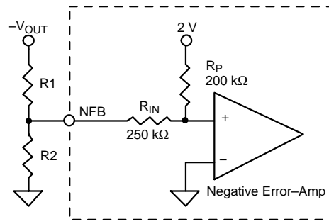
Figure 9. Negative Error Amplifier and NFB Pin
