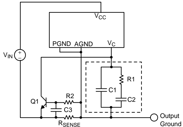
Figure 14. Current Limiting using a Current Sense Resistor
