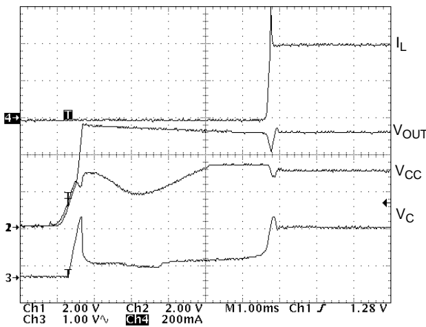
Figure 6. Startup Waveforms of Circuit Shown in the Application Diagram. Load = 400 mA.
