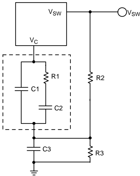
Figure 15. Technique for Increasing Slope Compensation
