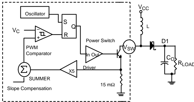
Figure 3. Current Mode Control Scheme
