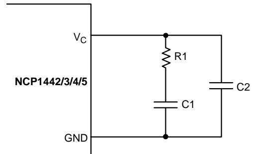
Figure 7. A Typical Compensation Network
