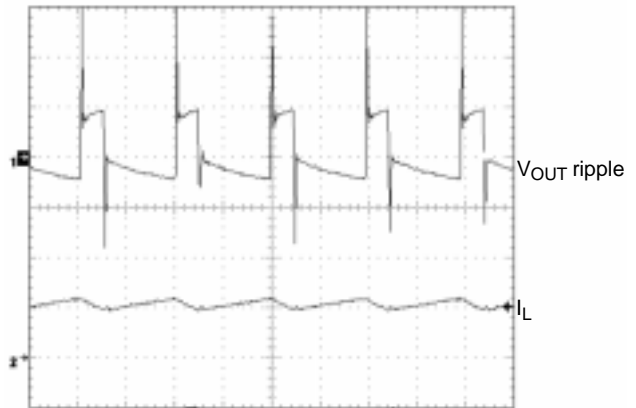
Figure 12. Typical Output Voltage Ripple
