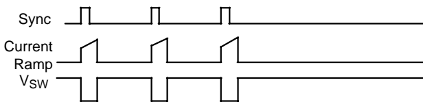
Figure 4. Timing Diagram of Sync and Shutdown
