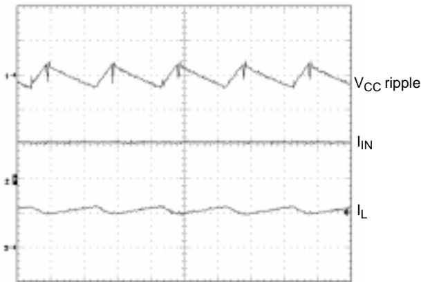
Figure 10. Boost Input Voltage and Current Ripple Waveforms
