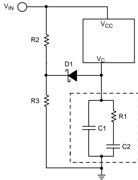
Figure 13. Current Limiting using a Diode Clamp
