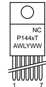
7 LEAD, TO-220
