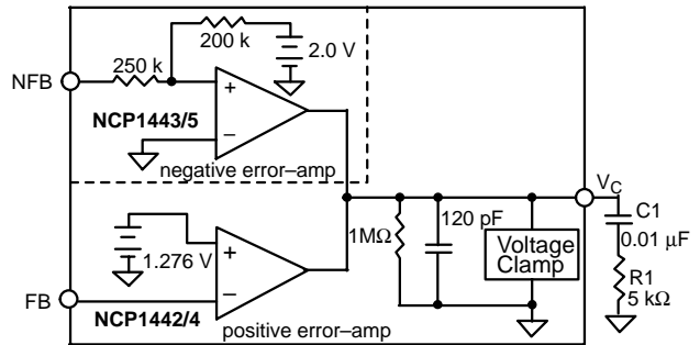
Figure 5. Error Amplifier Equivalent Circuit
