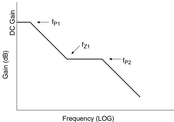
Figure 8. Bode Plot of the Compensation Network Shown in Figure 7
