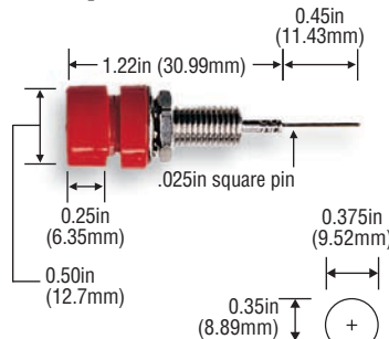
Panel Cut-Out
