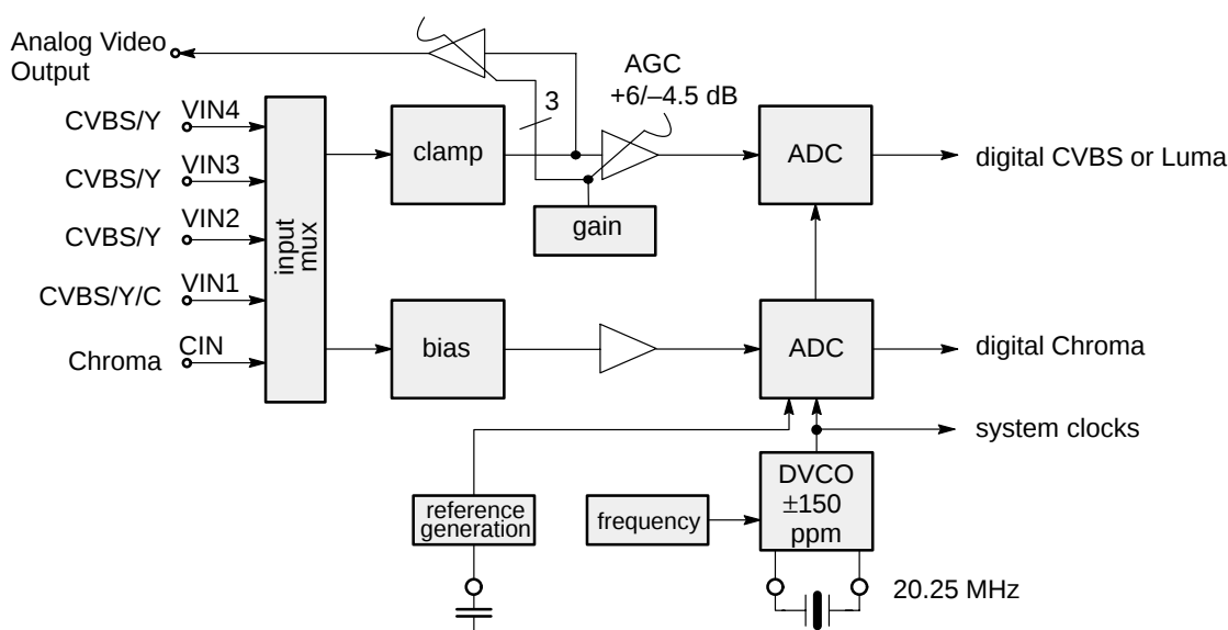
Fig. 2–1: Analog front-end
