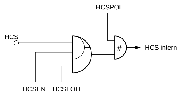
Fig. 2–26: Half Contrast Switch Logic
