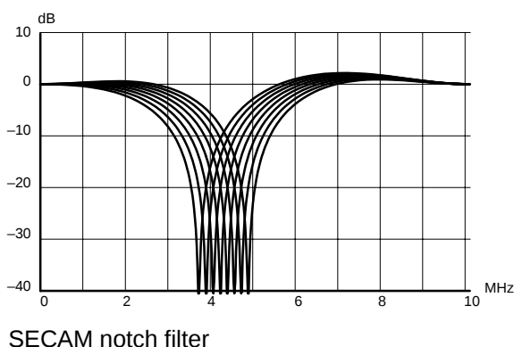
Fig. 2-10: Frequency responses of the luma notch filter for PAL, NTSC, and SECAM
