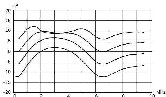
Fig. 2–15: Dynamic peaking frequency response
