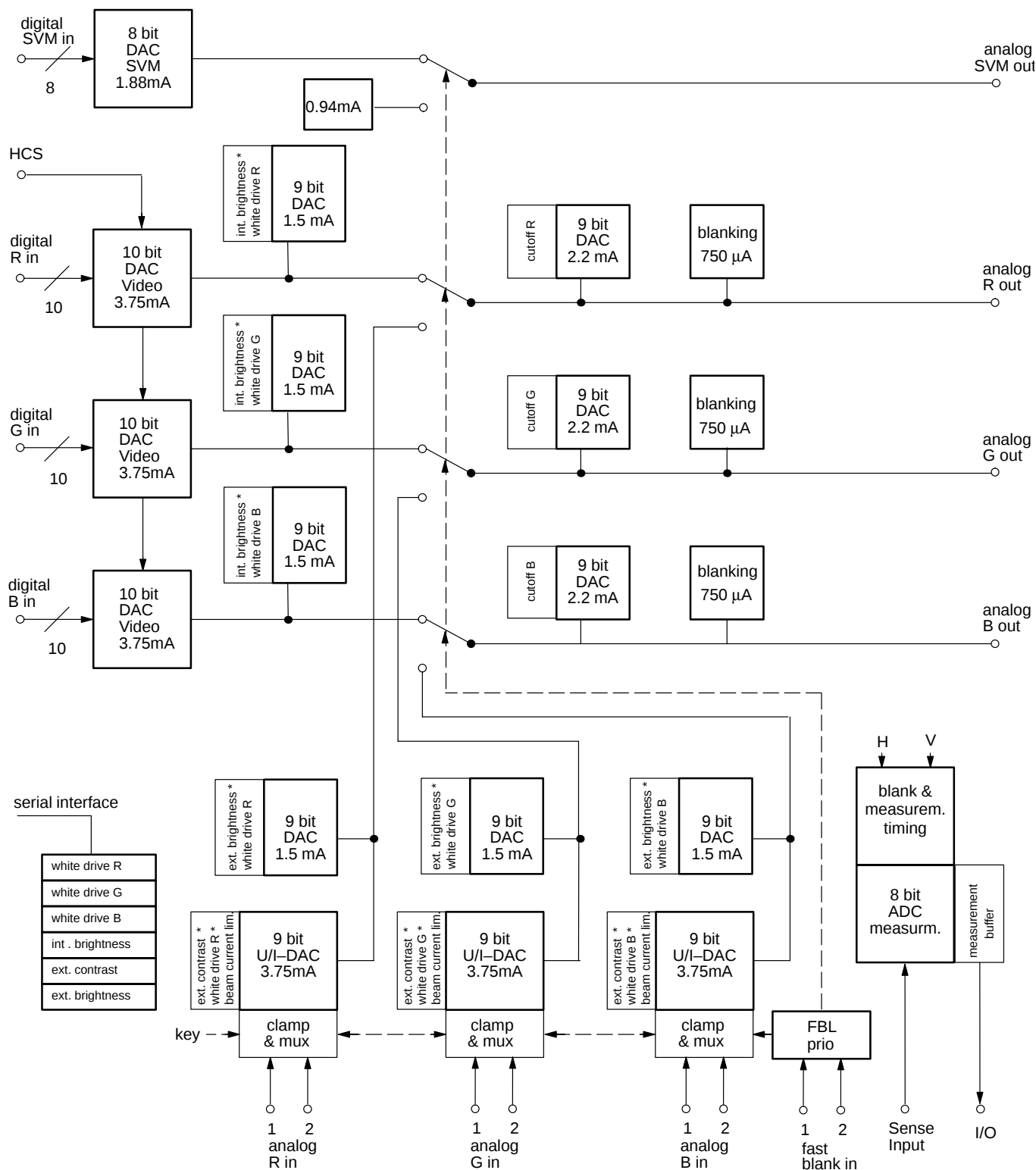
Fig. 2-27: Analog back-end
