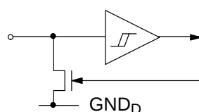
Fig. 4-12: Pins SDA, SCL
