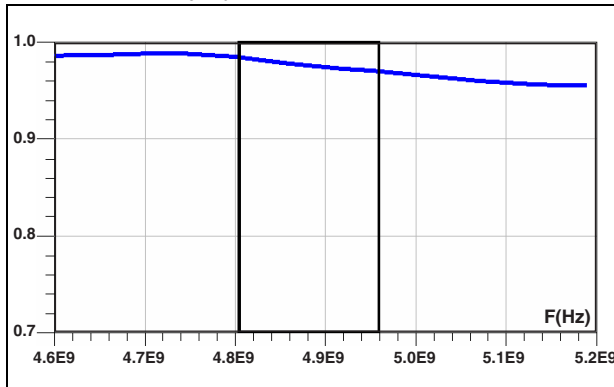
Figure 7. S_{cc22} magnitude @ 2f_0 ( T_{amb} = 25\text{ }^{\circ}\text{C} )
