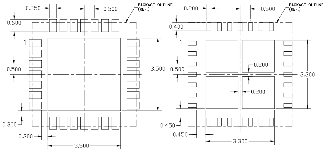
PCB SOLDER MASK TOP (X-RAY) VIEW
