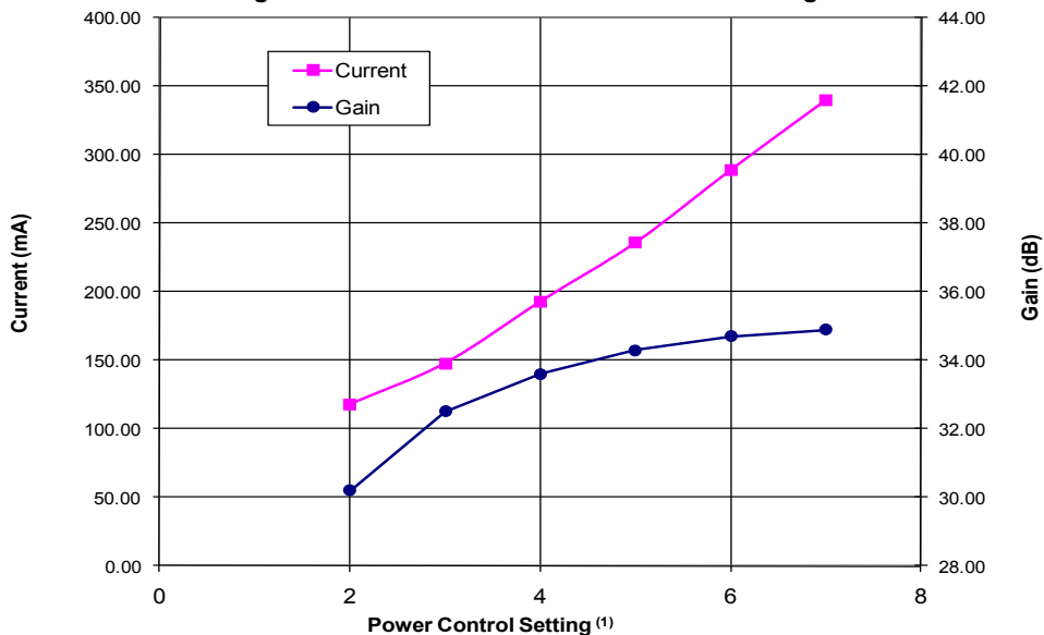
Figure 13: Gain &amp; Idd vs. Power Control Setting
