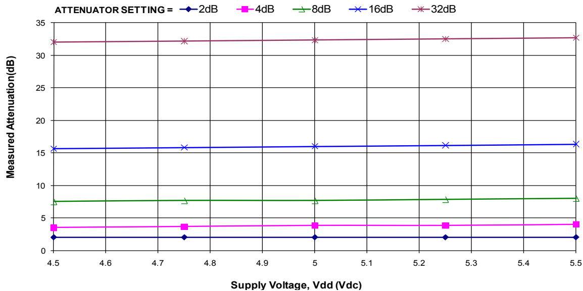
Figure 11: Attenuator Accuracy over Voltage ( T_c = +25^\circ\text{C} , F1 = 10\text{ MHz} )
