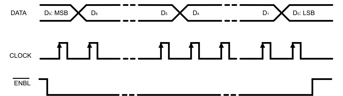
Figure 18: Serial Data Input Timing
