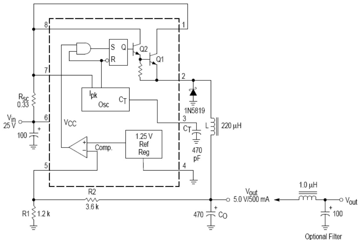
Figure 9. Step-Down Converter
