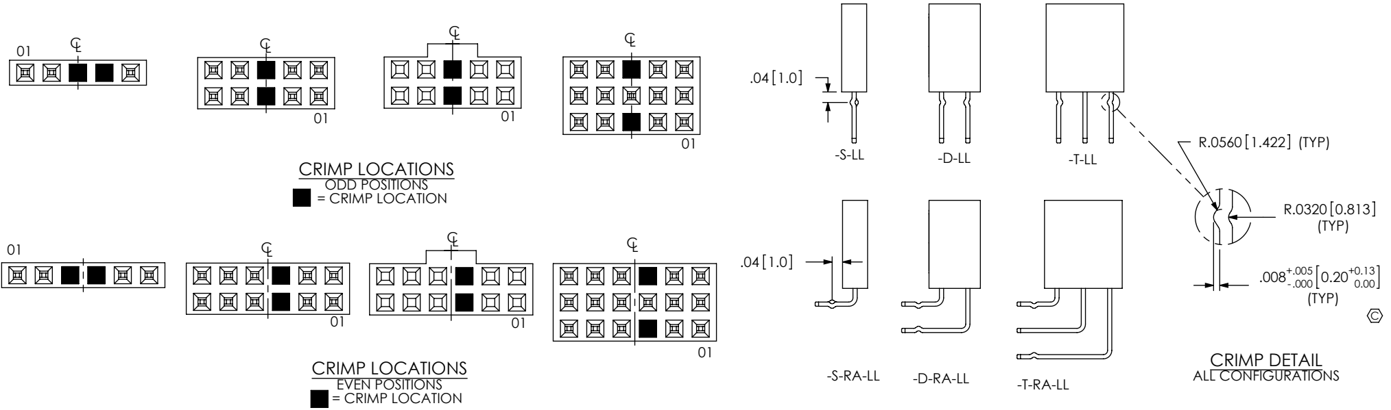
FIG 2 RIGHT ANGLE OPTION ALL OPTIONS DIFFERENT AS SHOWN, OTHERWISE SAME AS -S-RA
