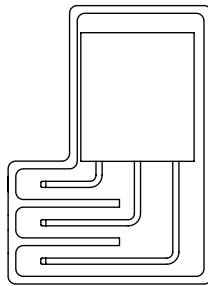
SSW-1XX-02-XXX-T-RA SSW-1XX-02-XXX-Q-RA
