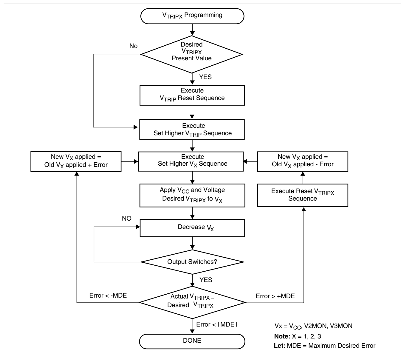
Figure 6. V_{TRIP} Set/Reset Sequence (X = 1, 2, 3)
