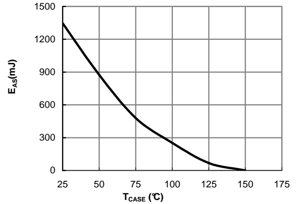
Figure 14: Avalanche energy
