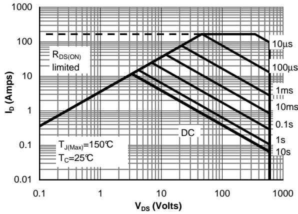
Figure 13: Maximum Forward Biased Safe Operating Area for AOTF42S60L(Note F)
