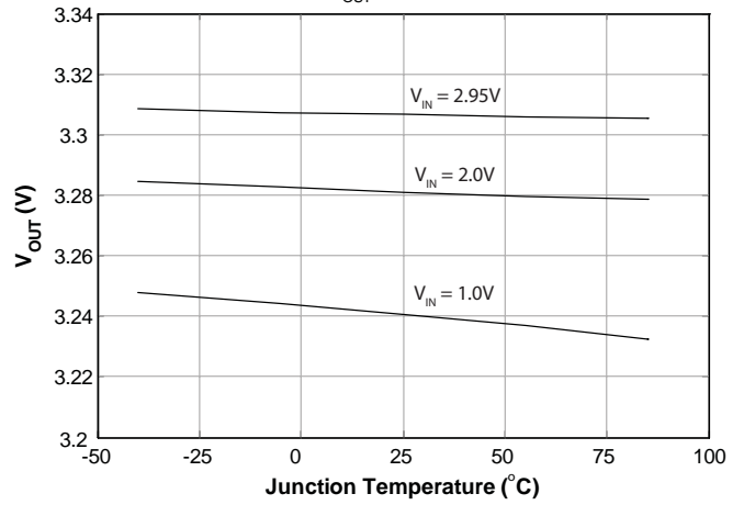
Temperature Reg. — High Load ( V_{OUT} = 3.3V )
