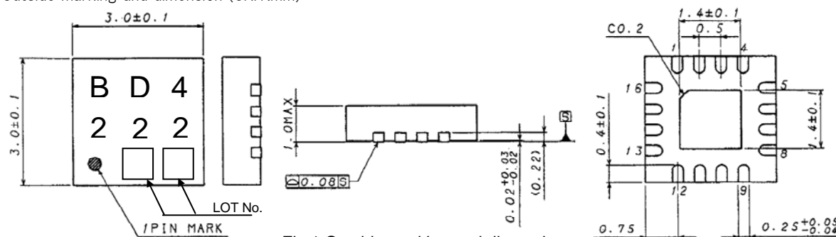
Fig.1 Outside marking and dimension
