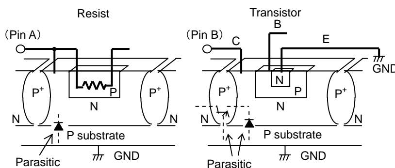
Fig.5 Other adjacent elements
