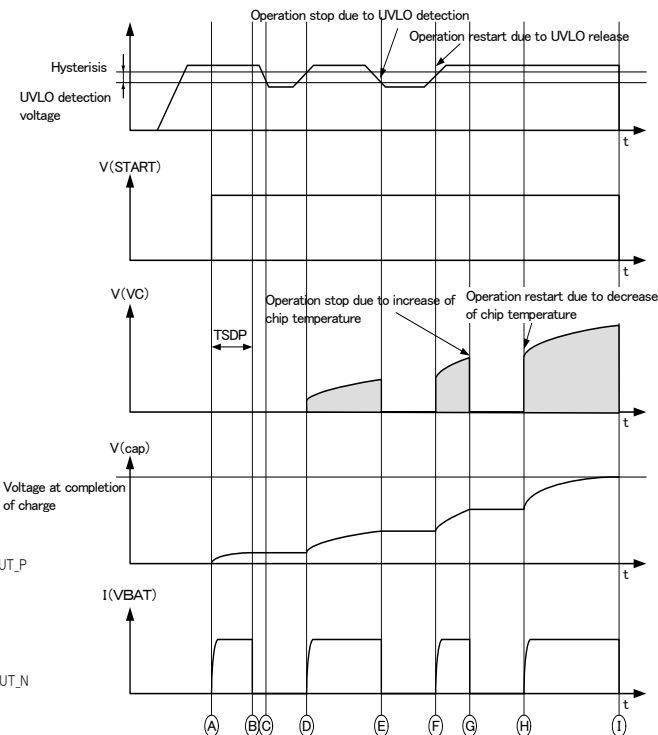
Fig.4 Timing Chart: Under Protective Circuit Operation
