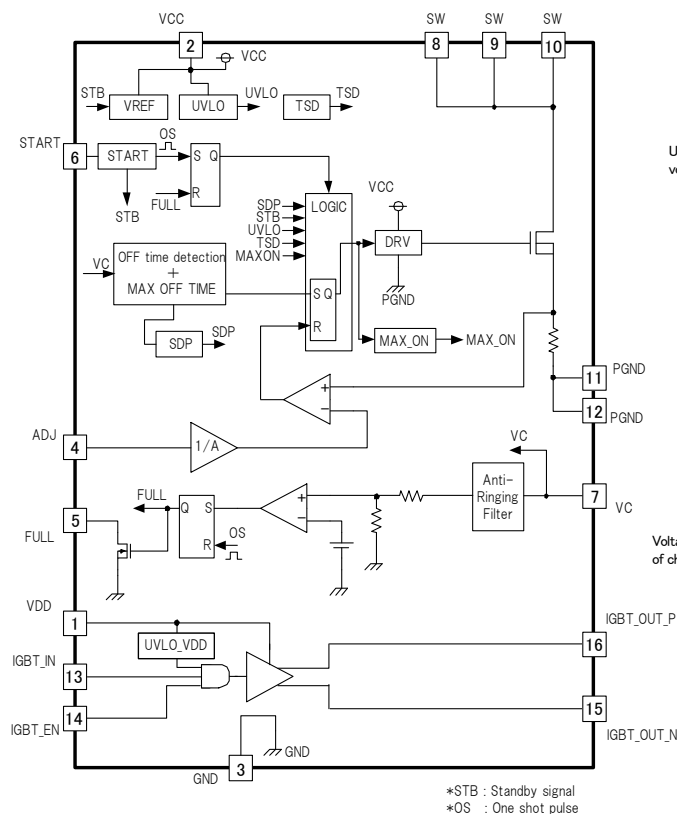
Fig.3 Block diagram
