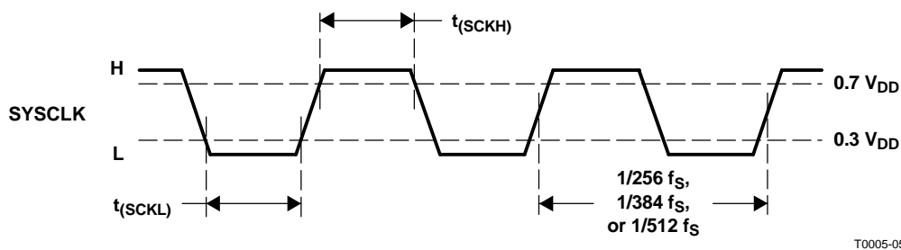
Figure 44. System Clock Timing
