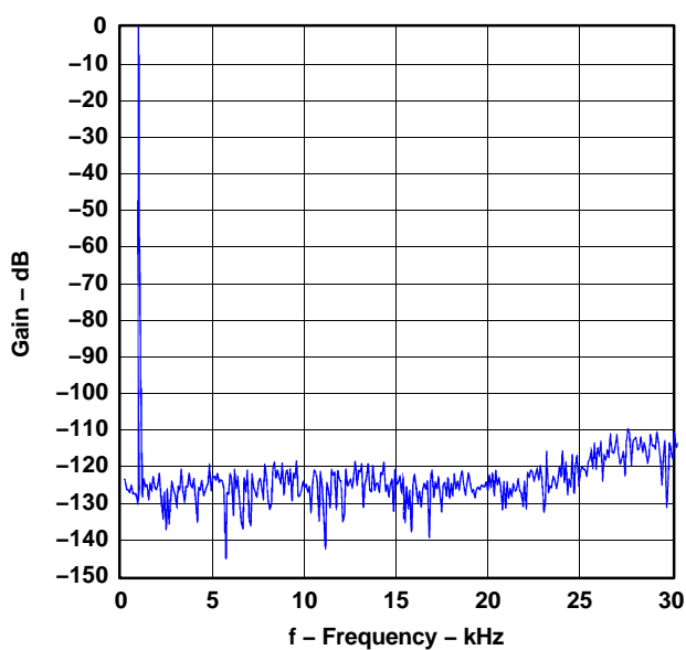
Figure 54. Quantization Noise Spectrum
