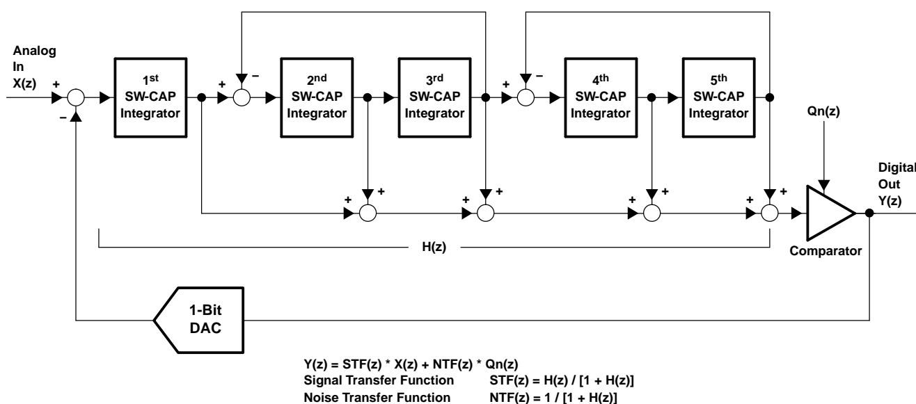
Figure 52. Simplified Fifth-Order Delta-Sigma Modulator
