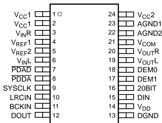
PCM3003 (TOP VIEW)
