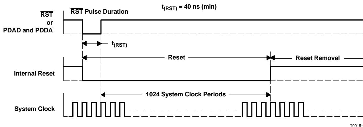
Figure 47. External Forced-Reset Timing
