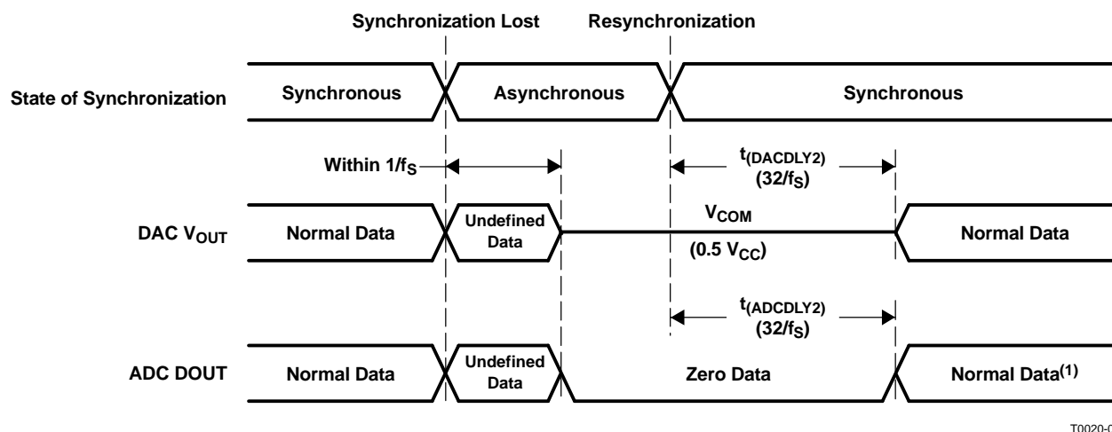
Figure 48. DAC Output and ADC Output for Loss of Synchronization
