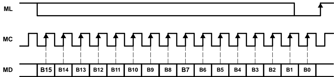
Figure 49. Control Data Input Format
