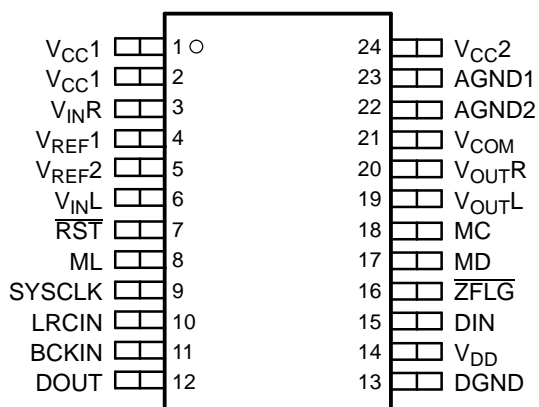
PCM3002 (TOP VIEW)
