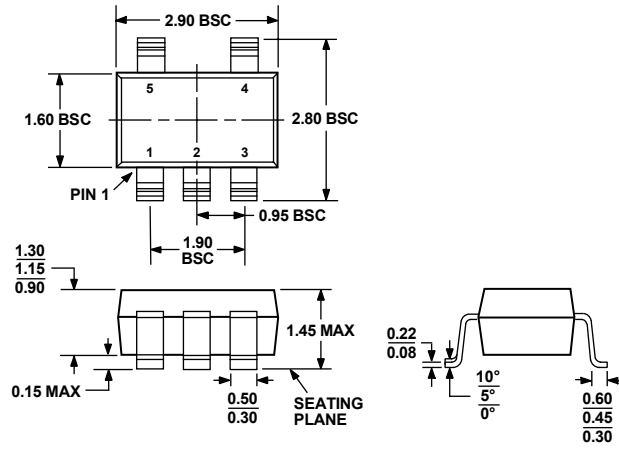
Figure 45. 5-Lead Small Outline Transistor Package [SOT-23]
