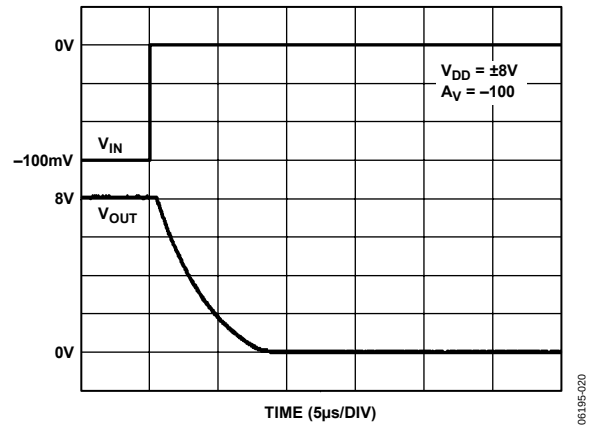
Figure 22. Positive Overload Recovery Time
