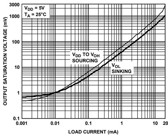
Figure 27. Output Saturation Voltage vs. Load Current
