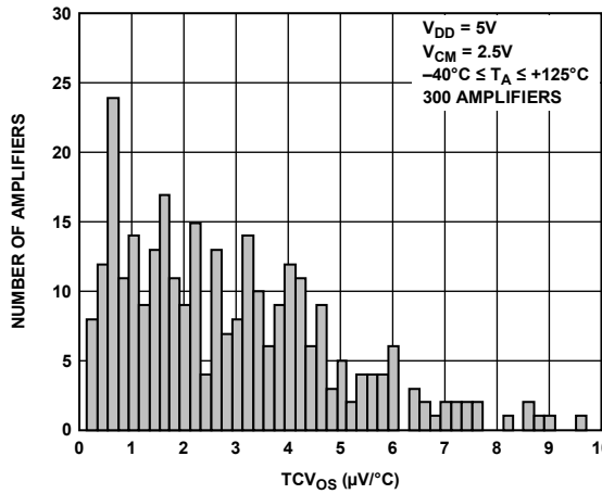
Figure 25. V_{OS} Drift ( TCV_{OS} ) Distribution
