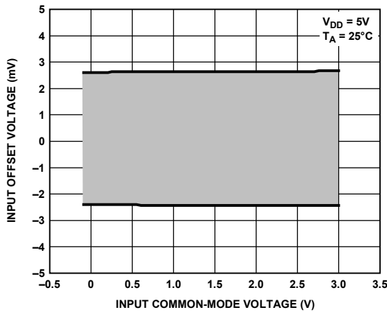
Figure 26. Offset Voltage vs. Common-Mode Voltage
