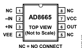
Figure 2. AD8665, 8-Lead SOIC_N (R-8)
