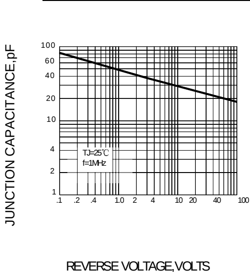
FIG.3-TYPICAL JUNCTION CAPACITANCE
