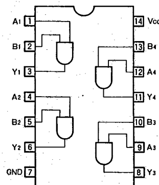
Fig. 21 BU74HC08
