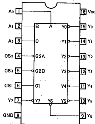
Fig. 36 BU74HC138
