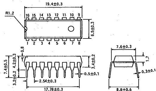
Fig. 2 16-pin DIP
