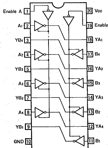
Fig. 43 BU74HC240
