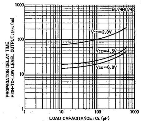
Fig. 18 High-to-low propagation delay time vs. load capacitance
