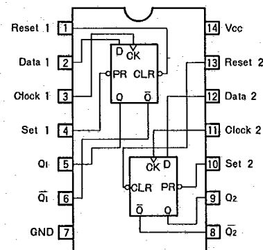
Fig. 29 BU74HC74
