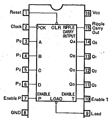
Fig. 40 BU74HC162
