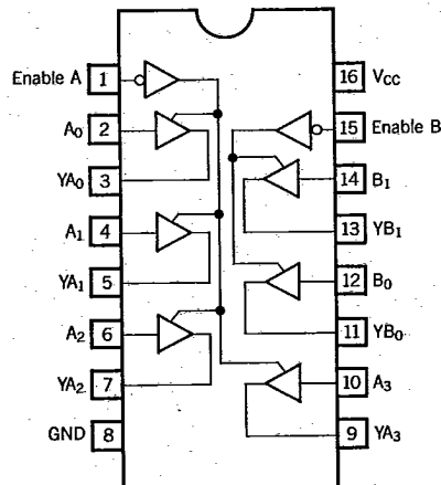
Fig. 46 BU74HC367
