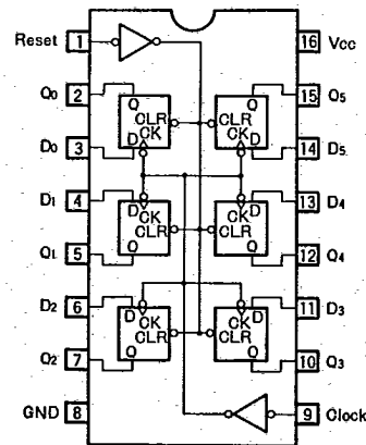
Fig. 31 BU74HC174
