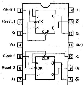
Fig. 28 BU74HC73
