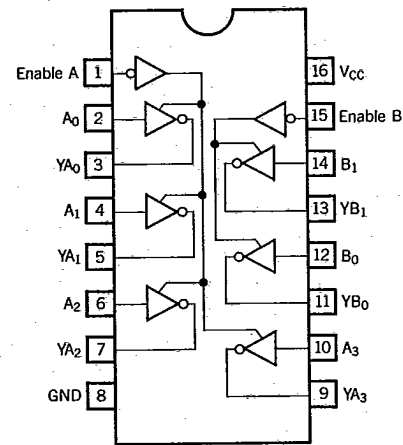
Fig. 47 BU74HC368
