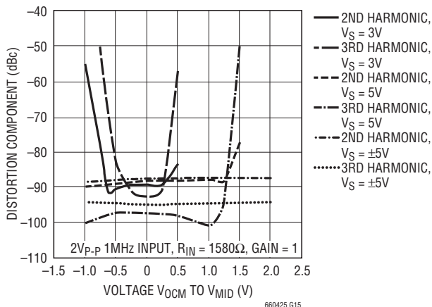
Distortion vs Output Common Mode Level
