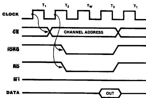
Figure 5. Read Cycle
