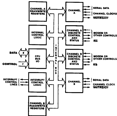
Figure 3. Block Diagram
