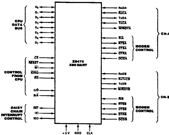
Figure 1. Pin Functions
