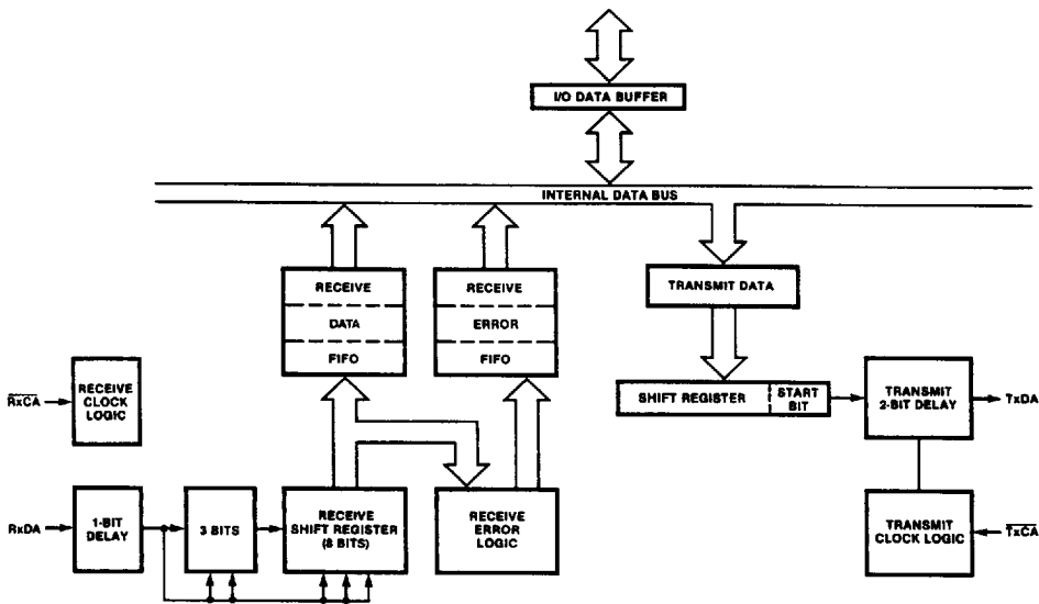
Figure 4. Data Path
