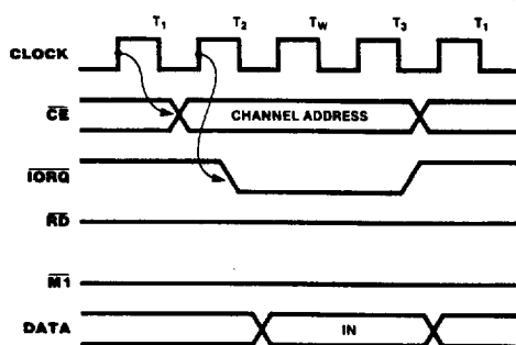
Figure 6. Write Cycle
