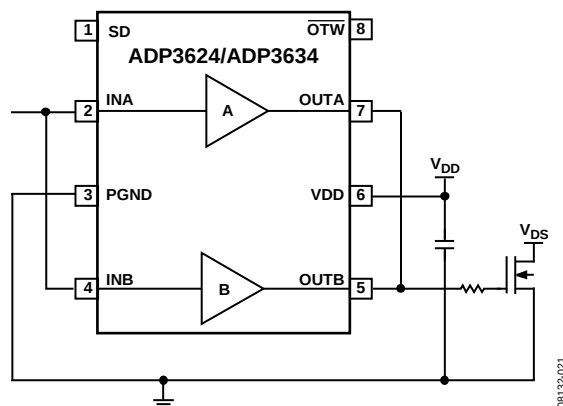
Figure 25. Parallel Operation
