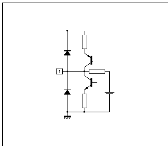
Figure 3 : CVBS Output
