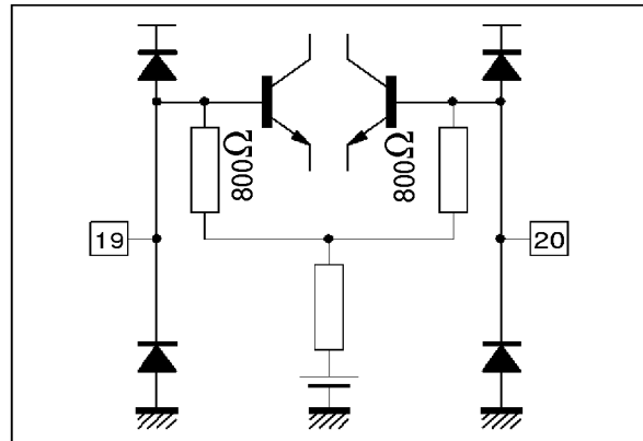
Figure 18 : AGC Capacitor
