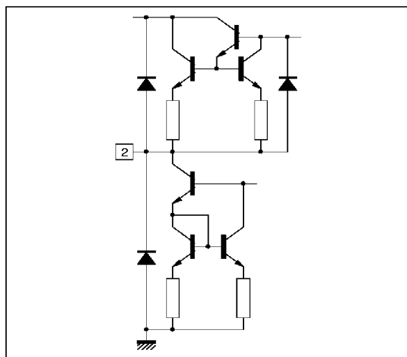
Figure 4 : Switching Input Standard + INT/EXT
