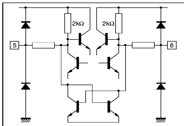
Figure 5 : IFLC
