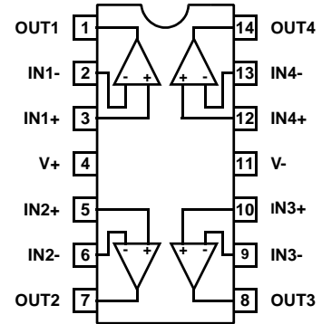
EL2444 [14-PIN SO (0.150"), PDIP] TOP VIEW
