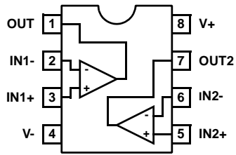
EL2244 (8-PIN SO, PDIP) TOP VIEW
