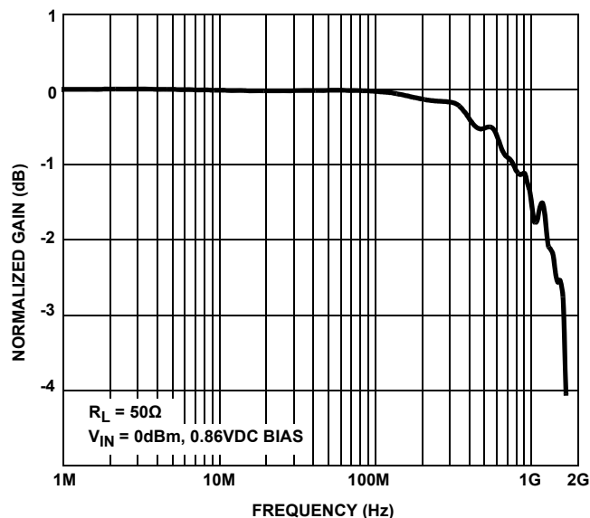
FIGURE 19. FREQUENCY RESPONSE
