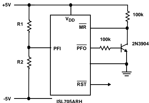
FIGURE 16. \pm 5V MONITORING
