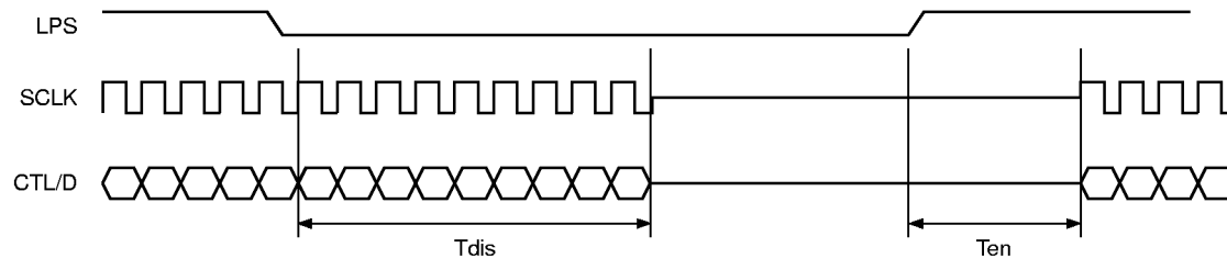
Fig. 3-2. LPS Timing
