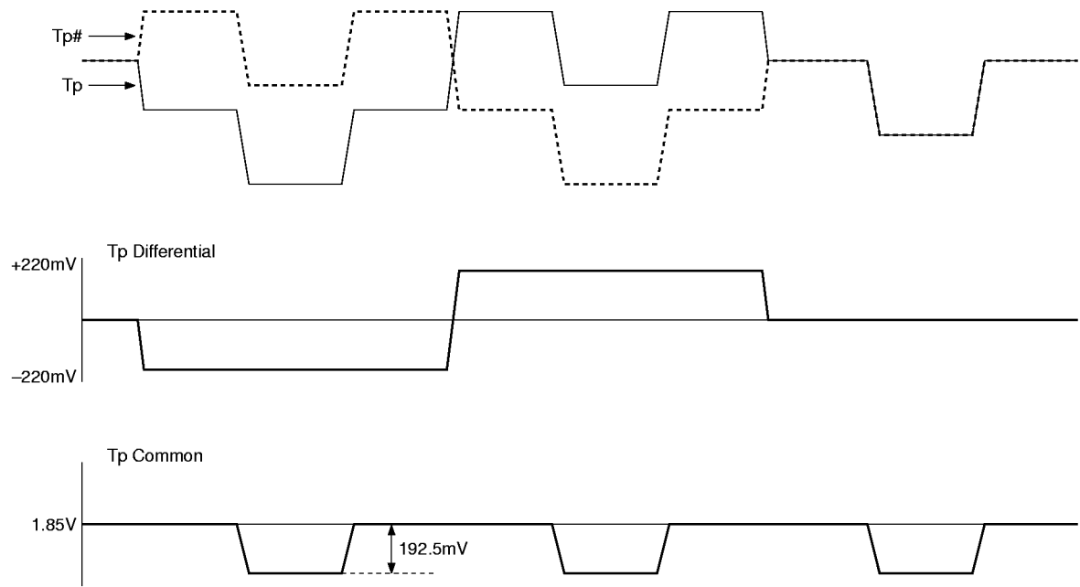
Fig. 3-10. Driver Current and Output Waveforms
