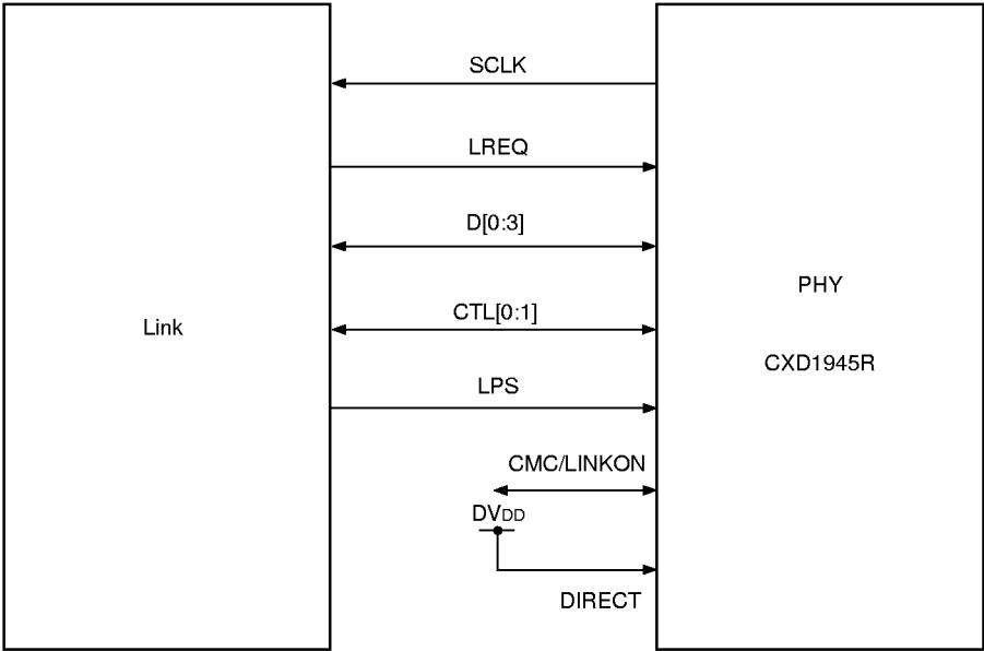
Fig. 3-1. CXD1945R – Link Chip Connection Diagram (DC Connection)
