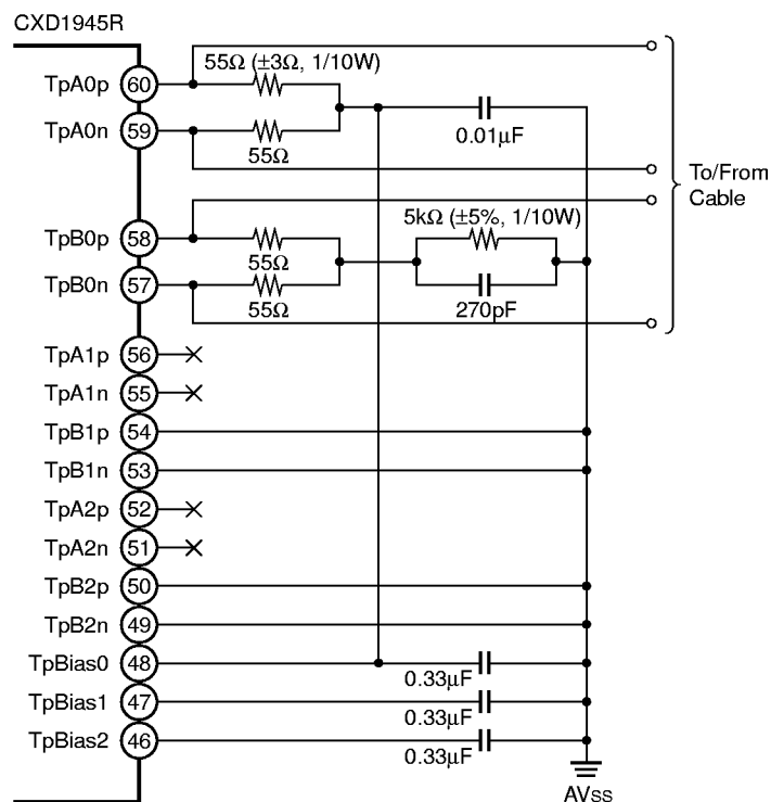
Fig. 3-11. Circuit Diagram when Using Only One Port
