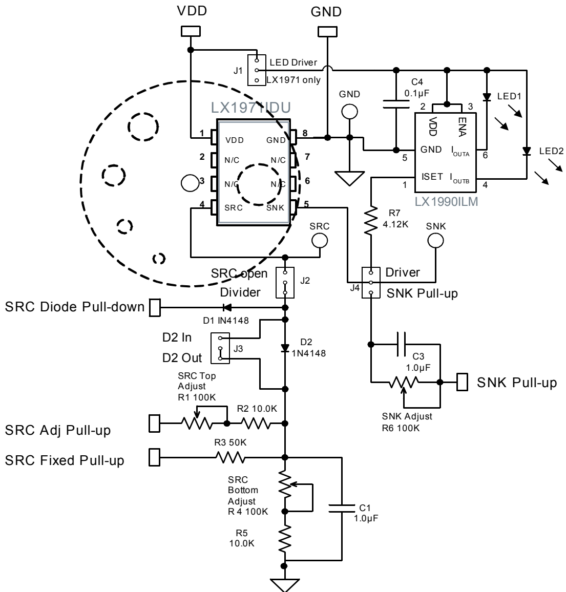
Figure 2 – Schematic
