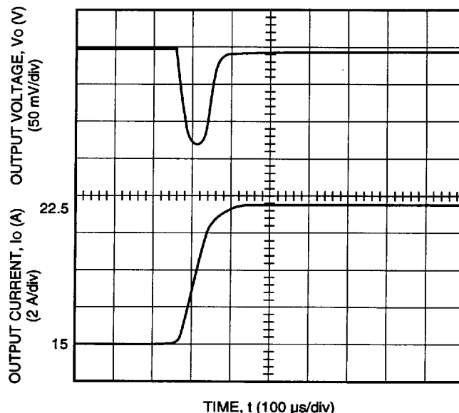
Figure 6. Typical FW150S4R0 Transient Response to Step Increase in Load from 50% to 75% of Full Load at Room Temperature and 54 V Input (Waveform Averaged to Eliminate Ripple Component.)
