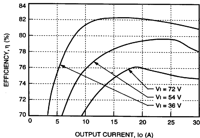
Figure 3. Typical FW150S4R0 Efficiency vs. Output Current at Room Temperature
