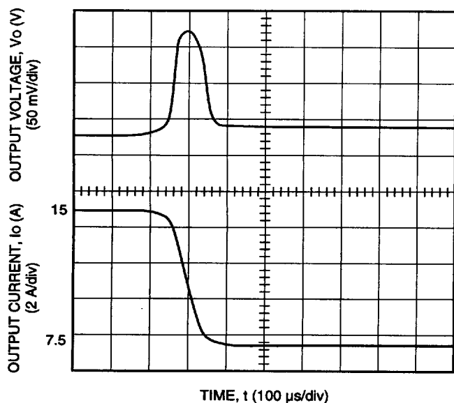
Figure 5. Typical FW150S4R0 Transient Response to Step Decrease in Load from 50% to 25% of Full Load at Room Temperature and 54 V Input (Waveform Averaged to Eliminate Ripple Component.)
