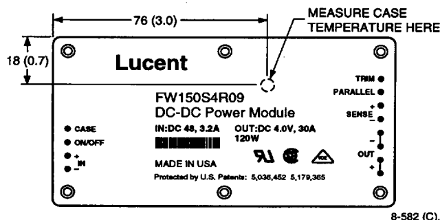
Figure 17. Case Temperature Measurement Location
