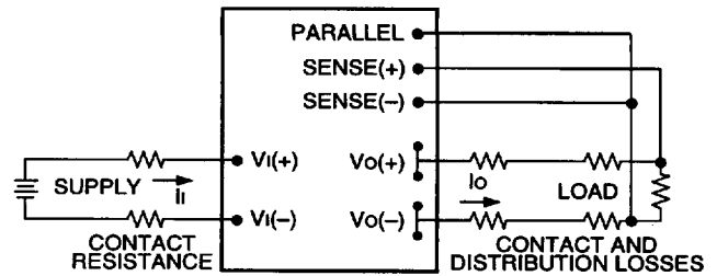
Figure 12. Effective Circuit Configuration for Single-Module Remote-Sense Operation
