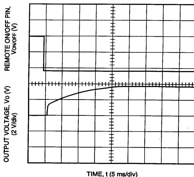
Figure 7. Typical FW150S4R0 Start-Up Transient at Room Temperature, 54 V Input, and 30 A Output
