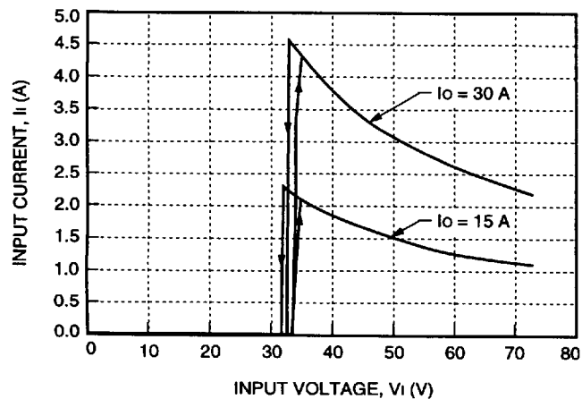
Figure 1. Typical FW150S4R0 Input Characteristics at Room Temperature
