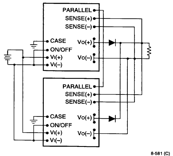
Figure 16. Wiring Configuration for Redundant Parallel Operation
