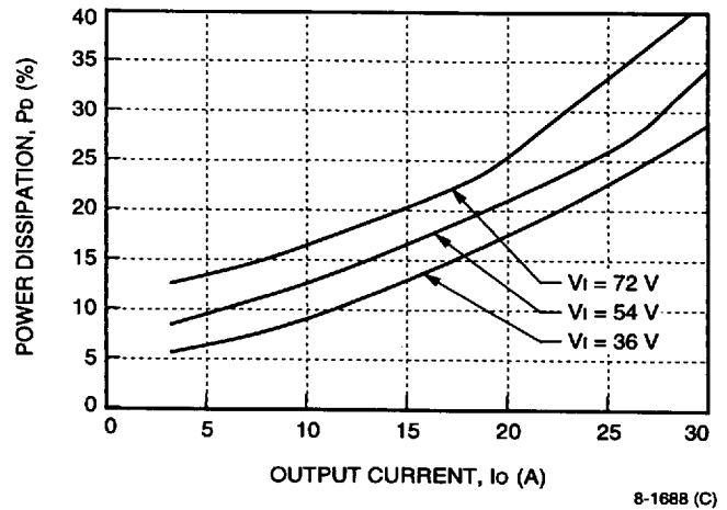
Figure 21. Power Dissipation as Heat vs. Output Current
