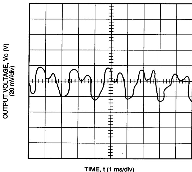
Figure 4. Typical FW150S4R0 Output Ripple Voltage at Room Temperature, 54 V Input, and 30 A Output
