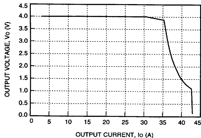
Figure 2. Typical FW150S4R0 Output Characteristics at Room Temperature and 54 V Input
