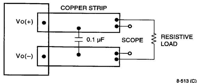
Figure 10. Peak-to-Peak Output Noise Measurement Test Setup
