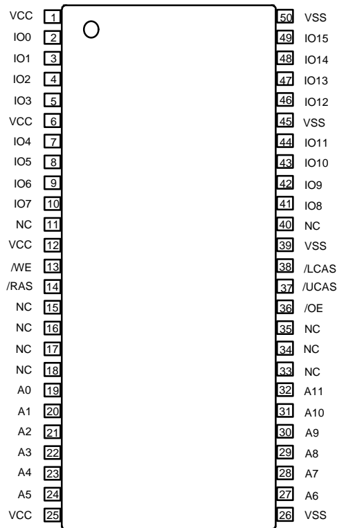
50 Pin Plastic SOJ / TSOP-II
