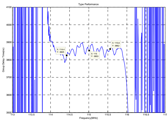
Group Delay Variation( f_0 \pm 0.6 MHz)
