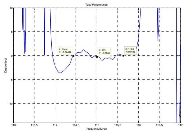
Phase Linearity( f_0 \pm 0.6 MHz)
