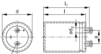
B43454 Ring clip/clamp mounting
