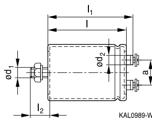
B43474 Threaded stud mounting
