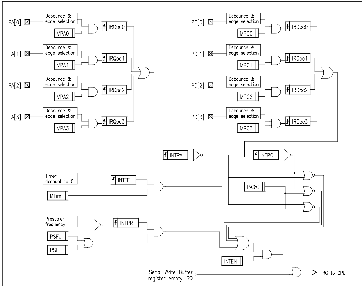
Figure 11.Interrupt Request generation
