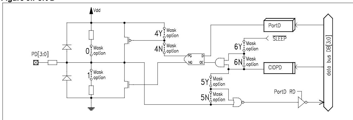
Figure 9. Port D
