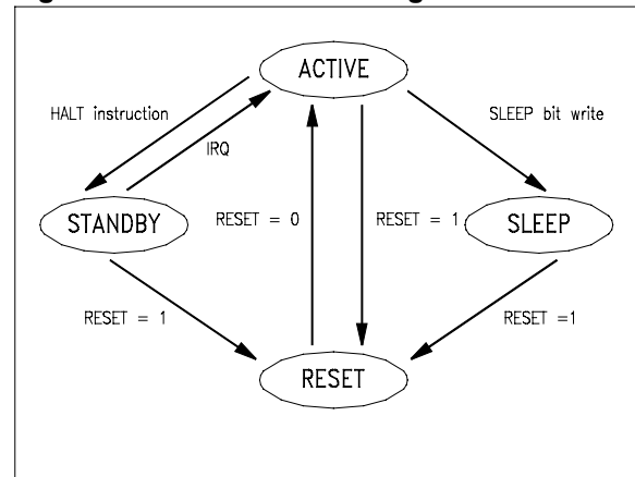
Figure 4. Mode Transition diagram
