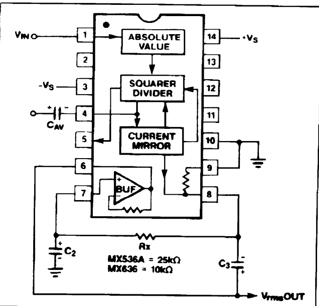
Figure 8. MX536A/MX636 with a 2 Pole Output Filter
