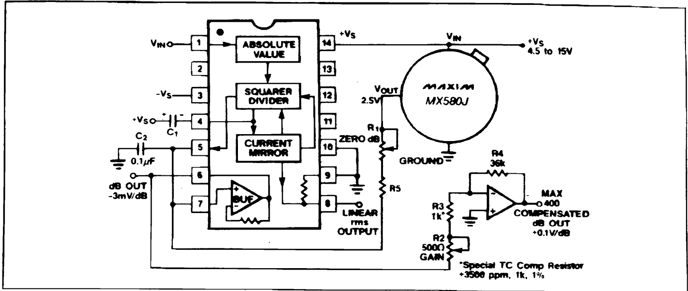
Figure 10. dB Connection
