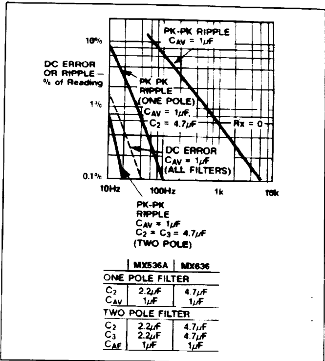
Figure 9. Performance Features of Various Filter Types for MX536A/MX636
