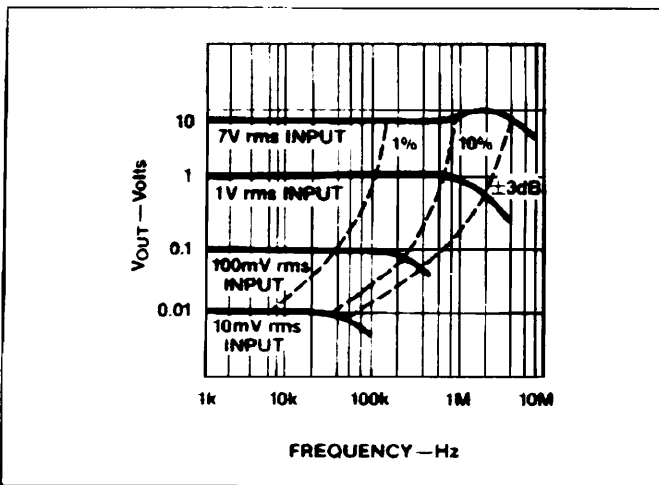
Figure 11. MX536A High Frequency Response
