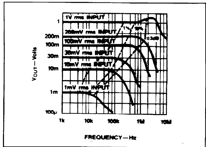
Figure 12. MX636 High Frequency Response
