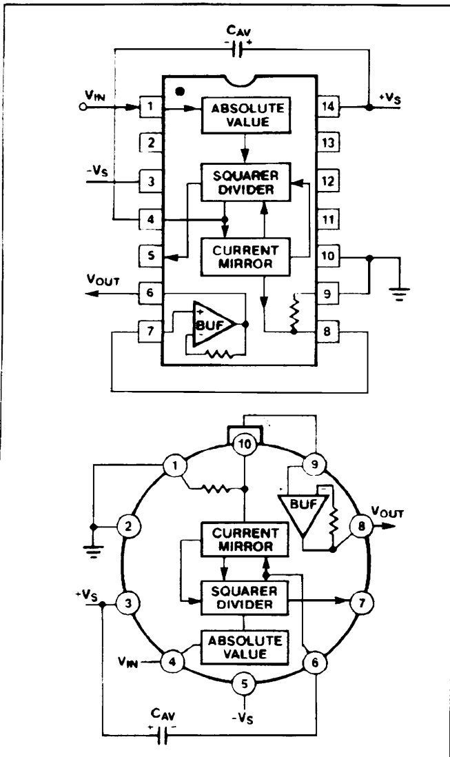
Figure 2. MX536A/MX636 Standard rms Connection
