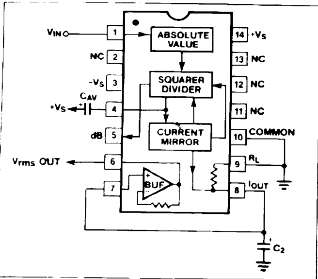
Figure 7. MX536A/MX636 with a 1 Pole Output Filter
