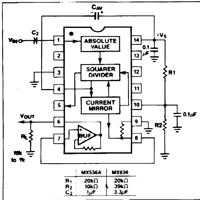
Figure 5. Single Supply Operation
