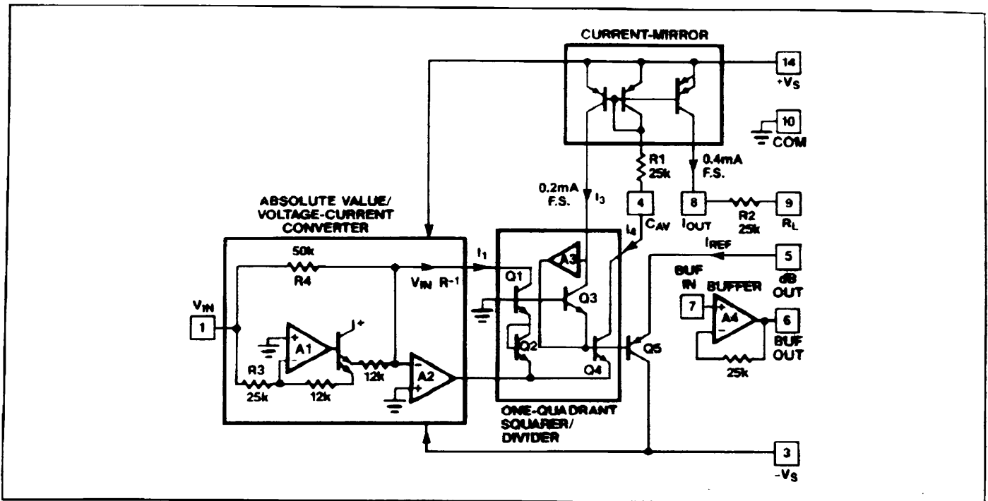
Figure 1. MX536A Simplified Schematic
