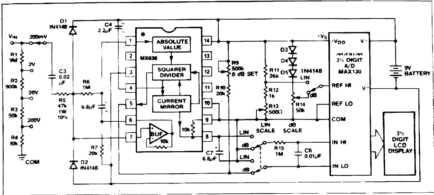
Figure 13. A Portable, High Z Input, rms DPM and dB Meter
