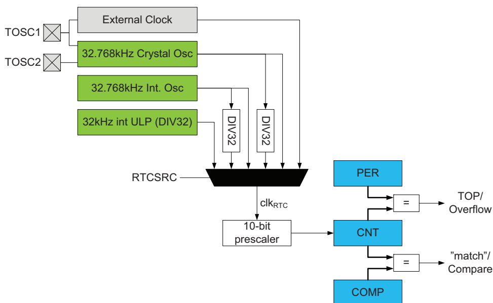
Figure 19-1. Real Time Counter overview
