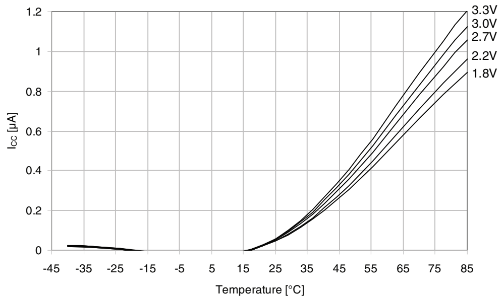
Figure 36-12. Power-down Supply Current vs. Temperature
