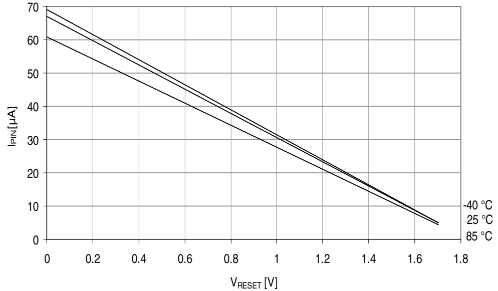
Figure 36-14. Reset and I/O Pull-up Resistor Current vs. Reset Pin Voltage V_{CC} = 1.8V
