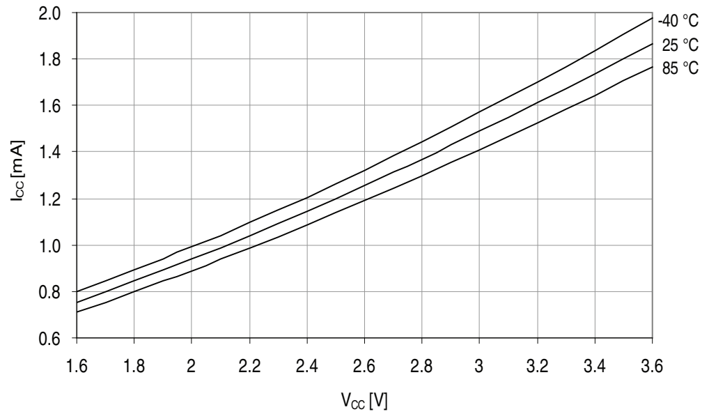
Figure 36-11. Idle Supply Current vs. V CC
