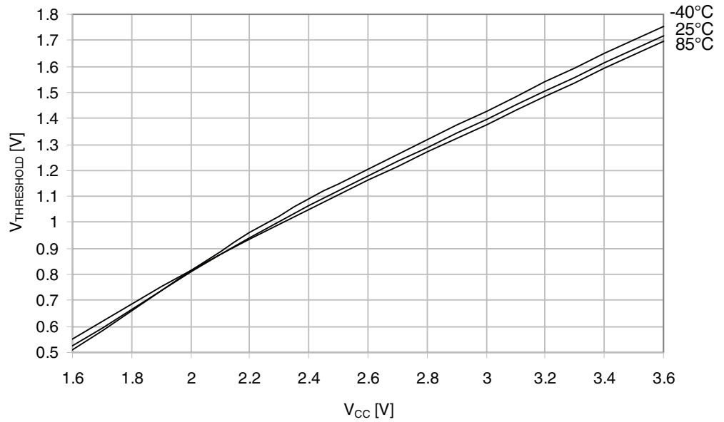
Figure 36-28. Reset Input Threshold Voltage vs. V_{CC}
