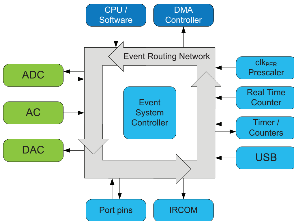
Figure 9-1. Event system block diagram
