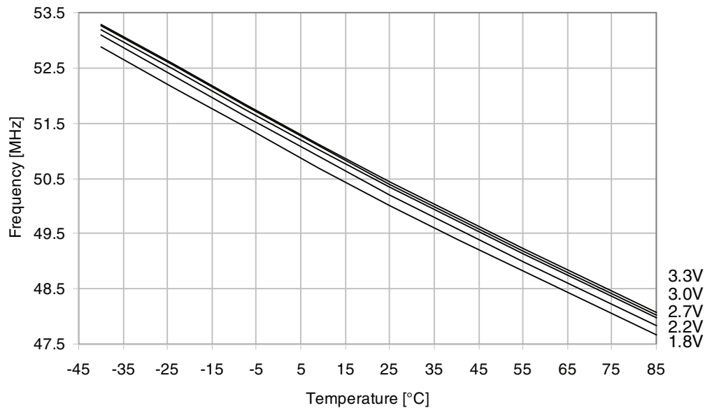
Figure 36-40. 48MHz Internal Oscillator Frequency vs. Temperature DPLL enabled, from 32.768kHz internal oscillator
