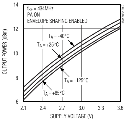
OUTPUT POWER vs. SUPPLY VOLTAGE MAX7032 toc29-2
