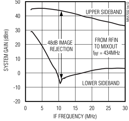
SYSTEM GAIN vs. IF FREQUENCY
