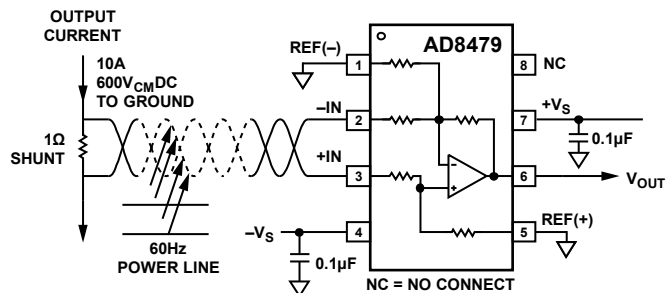
Figure 41. Error Budget Analysis Example: V_{IN} = 10\text{ V Full Scale} , V_{CM} = 600\text{ V DC} , R_{SHUNT} = 1\ \Omega , 1\text{ V p-p} , 60\text{ Hz Power Line Interference}
