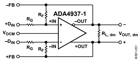
Figure 46. Circuit Definitions
