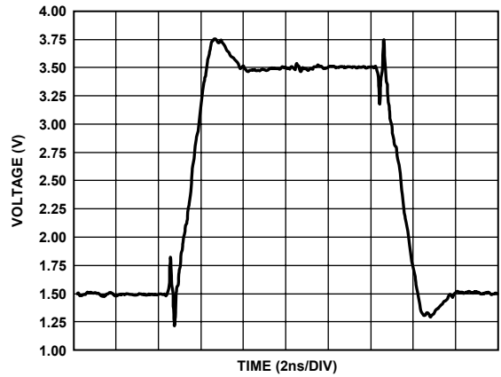
Figure 40. Large Signal V_{OCM} Pulse Response
