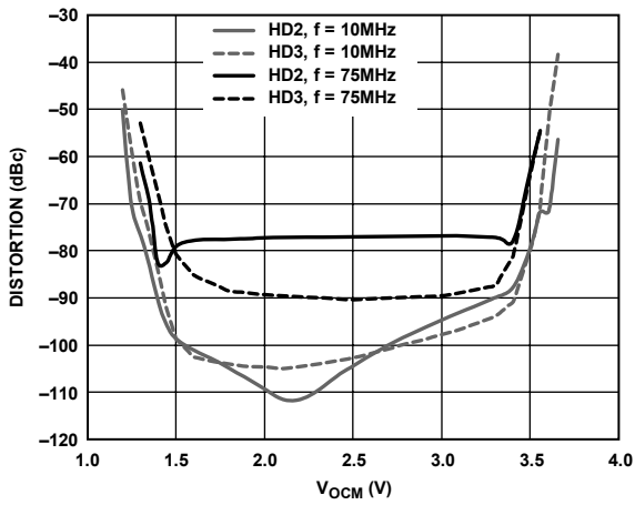
Figure 23. Harmonic Distortion vs. V_{OCM} and Frequency
