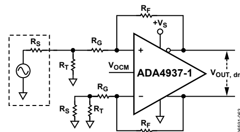
Figure 49. ADA4937-1 Configured for Unbalanced (Single-Ended) Input
