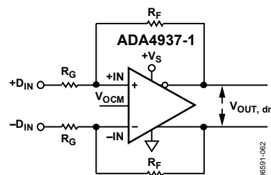
Figure 48. ADA4937-1 Configured for Balanced (Differential) Inputs
