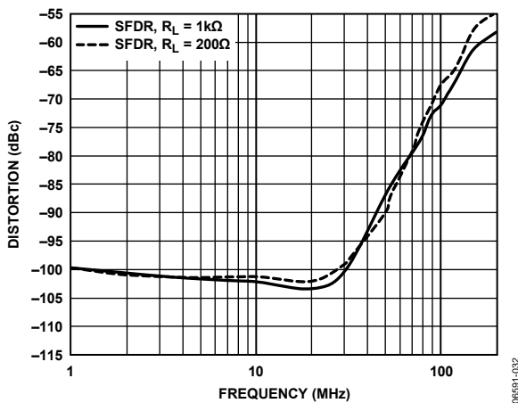
Figure 31. Spurious-Free Dynamic Range vs. Frequency and Load
