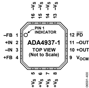
Figure 4. Pin Configuration
