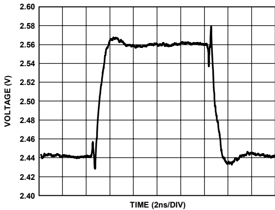
Figure 37. Small Signal V_{OCM} Pulse Response
