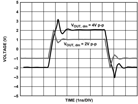
Figure 39. Large Signal Pulse Response
