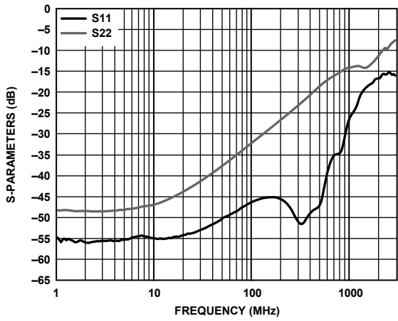
Figure 30. Return Loss ( S_{11} , S_{22} ) vs. Frequency
