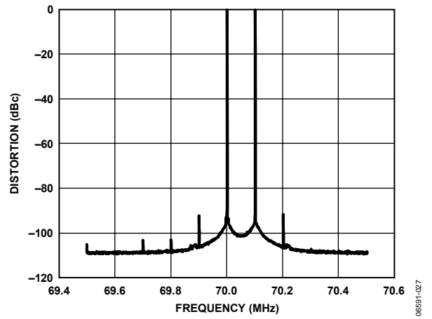
Figure 26. 70 MHz Intermodulation Distortion
