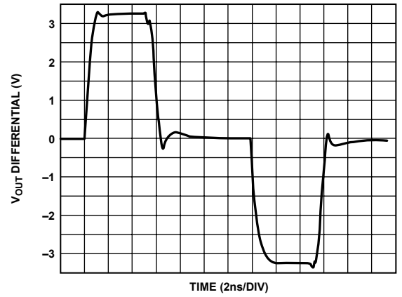
Figure 33. Overdrive Recovery Time (Pulse Input)
