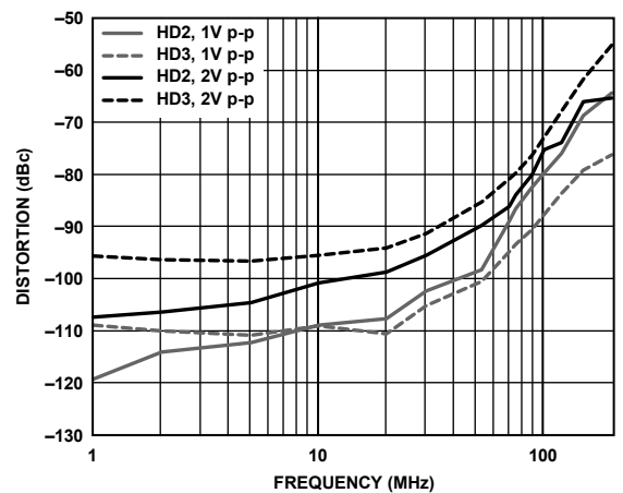
Figure 25. Harmonic Distortion vs. Frequency and V_{OU} , V_S = 3.3 V
