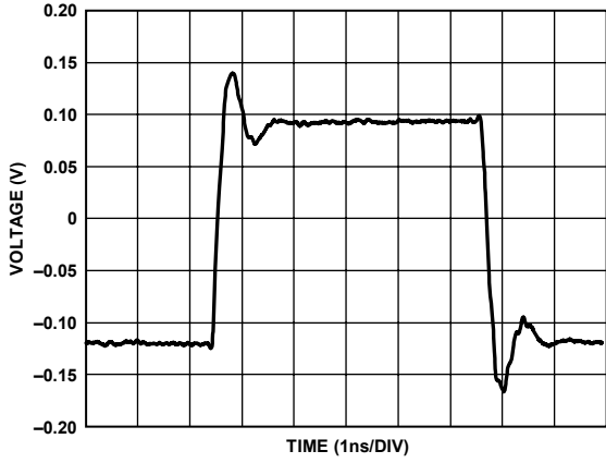
Figure 36. Small Signal Pulse Response
