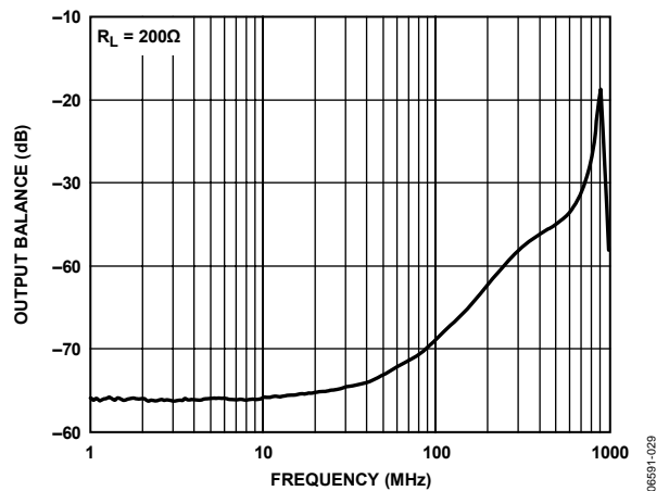
Figure 28. Output Balance vs. Frequency
