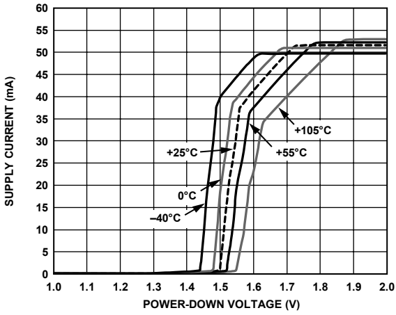
Figure 35. Supply Current vs. \overline{PD} for Various Temperatures
