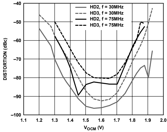
Figure 24. Harmonic Distortion vs. V_{OCM} and Frequency, V_S = 3.3 V
