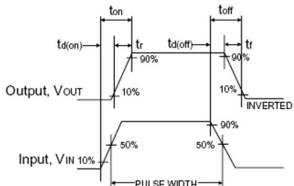
Switchin Waveforms
