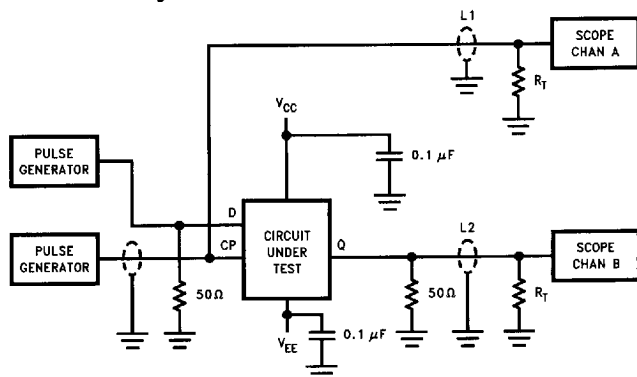
FIGURE 1. Toggle Frequency Test Circuit
