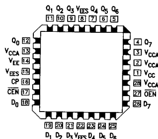
28-Pin PCC
