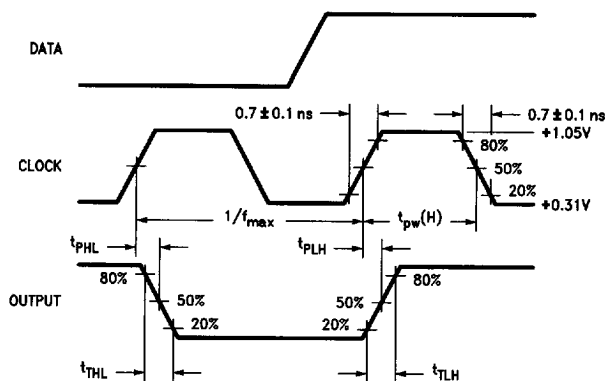
FIGURE 4. Propagation Delay (Clock) and Transition Times
