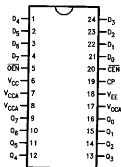
24-Pin DIP
