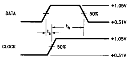
FIGURE 6. Data Setup and Hold Time
