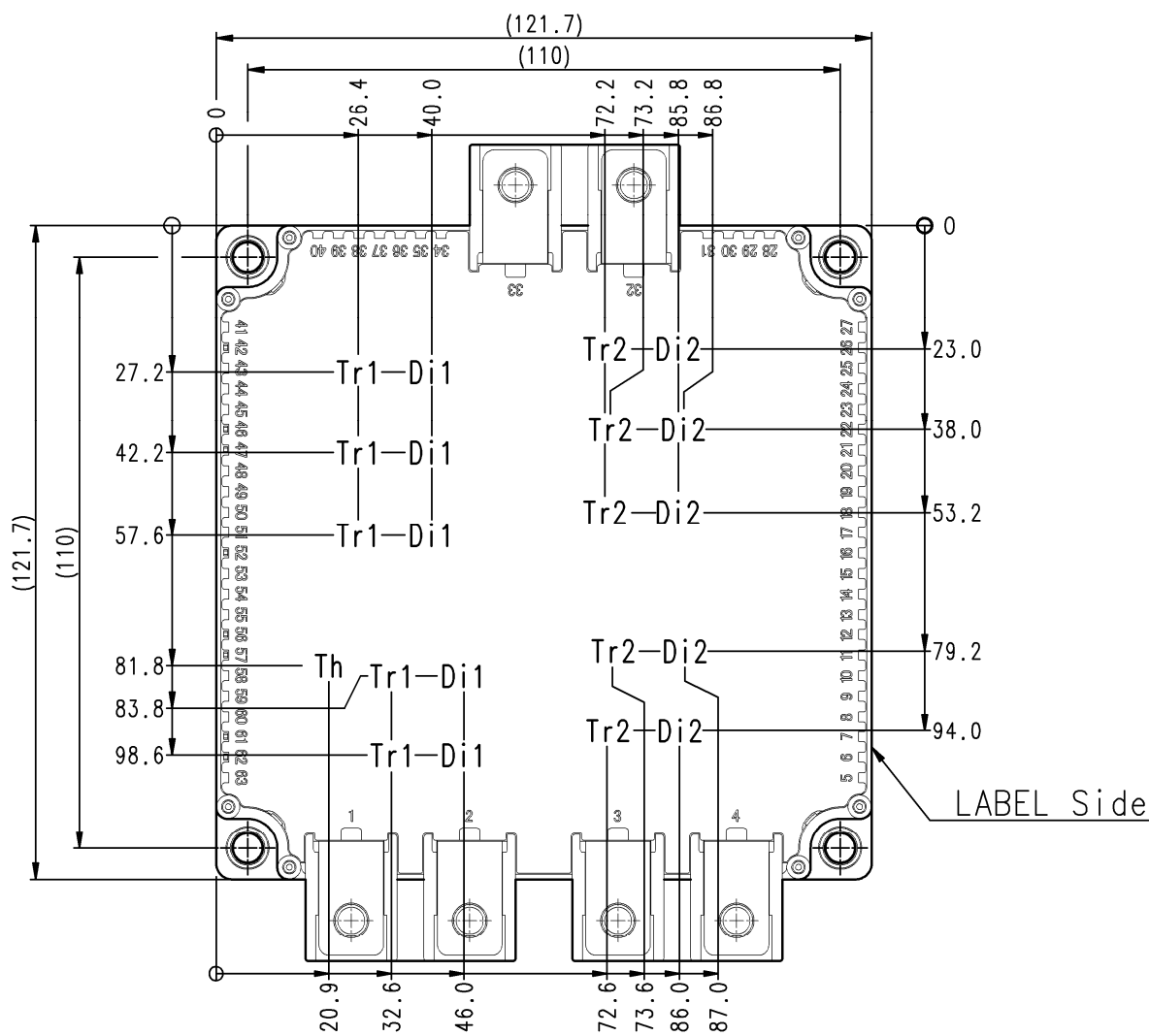
Tr1/Tr2: IGBT, Di1/Di2: FWDi, Th: NTC thermistor
