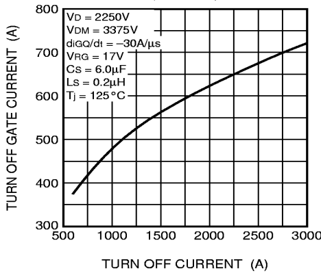
TURN OFF GATE CURRENT VS. TURN OFF CURRENT (TYPICAL)
