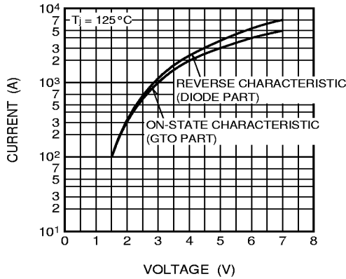
MAXIMUM ON-STATE AND MAXIMUM REVERSE CHARACTERISTICS
