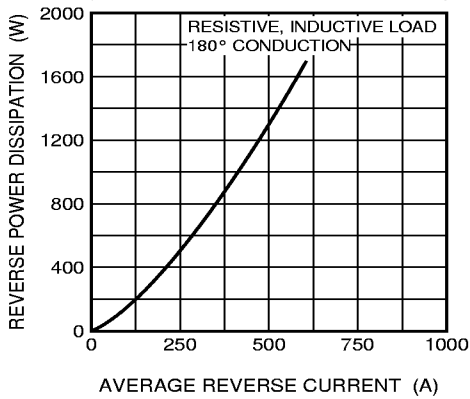
MAXIMUM REVERSE POWER DISSIPATION CHARACTERISTICS (DIODE PART, SINGLE PHASE WAVE)
