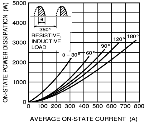
MAXIMUM ON-STATE POWER DISSIPATION CHARACTERISTICS (GTO PART, SINGLE-PHASE HALF WAVE)
