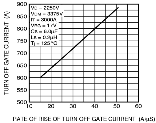
TURN OFF GATE CURRENT VS. RATE OF RISE OF GATE CURRENT (TYPICAL)
