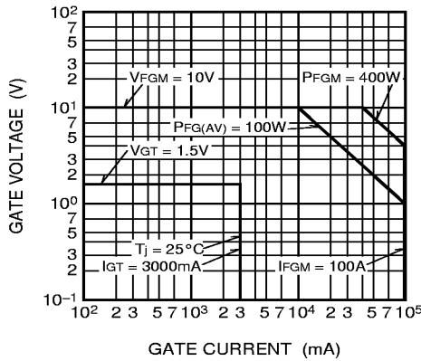
GATE CHARACTERISTICS
