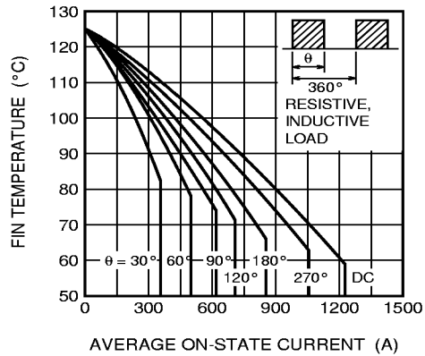
ALLOWABLE FIN TEMPERATURE VS. AVERAGE ON-STATE CURRENT (GTO PART, RECTANGULAR WAVE)
