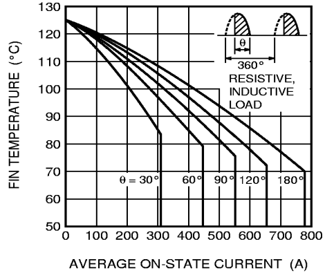
ALLOWABLE FIN TEMPERATURE VS. AVERAGE ON-STATE CURRENT (GTO PART, SINGLE-PHASE HALF WAVE)
