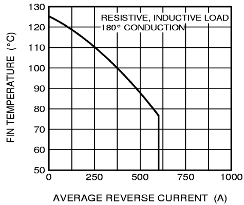
ALLOWABLE FIN TEMPERATURE VS. AVERAGE REVERSE CURRENT (DIODE PART, SINGLE PHASE HALF WAVE)
