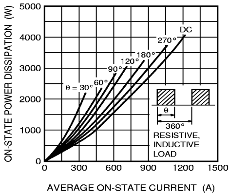
MAXIMUM ON-STATE POWER DISSIPATION CHARACTERISTICS (GTO PART, RECTANGULAR WAVE)
