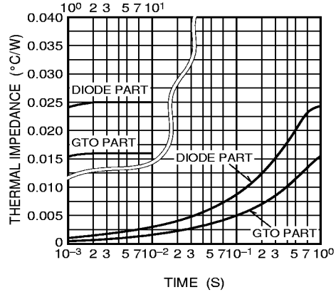
MAXIMUM THERMAL IMPEDANCE CHARACTERISTICS (JUNCTION TO FIN)
