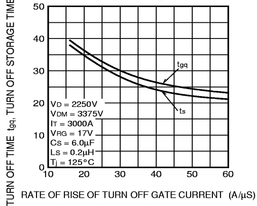
TURN OFF TIME, TURN OFF STORAGE TIME VS. RATE OF RISE OF TURN OFF GATE CURRENT (TYPICAL)
