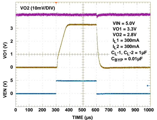
FIGURE 12. TURN-ON/TURN-OFF RESPONSE
