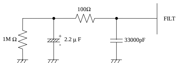
Figure 9 FILT recommended circuit
